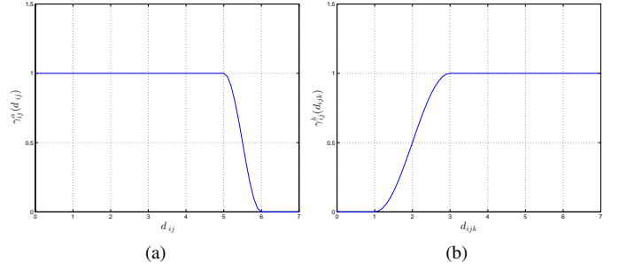
Fig. 3: The shape of \gamma_{ij}^a(d_{ij}) for d_1 = 5 , D = 6 , k_\gamma^a = 1 (a) and \gamma_{ij}^b(d_{ij,k}) for d_{\min}^o = 1 , d_{\max}^o = 3 , k_\gamma^b = 1 (b).
