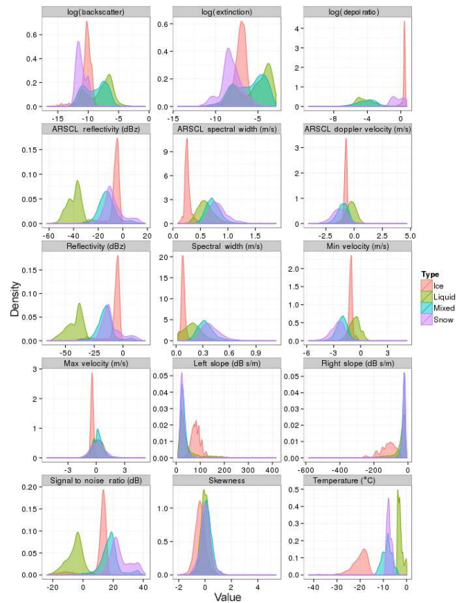
Figure 9. Histograms of algorithm training data set input variable values for four phase categories. Note that temperature is not included in the retrieval algorithm, but is included here for reference. Most clouds examined in this study are in the potentially mixed-phase temperature range ( -40 – 0 °C).
