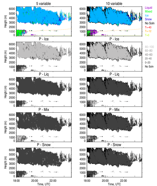
Figure 10. Application of 5-variable (left) and 10-variable (right) phase algorithms to 1 October 2004 test case. Color panels show algorithm identification when probability of a given phase is greater than 60 %. Gray-scale figures show probabilities of a given phase in percentage.
