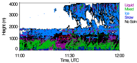
Figure 14. Phase identified by the 10-variable algorithm on 6 October 2004, 11:00–12:00 UTC; red box indicates region expected to be primarily drizzle based on study by Verlinde et al. (2013).
