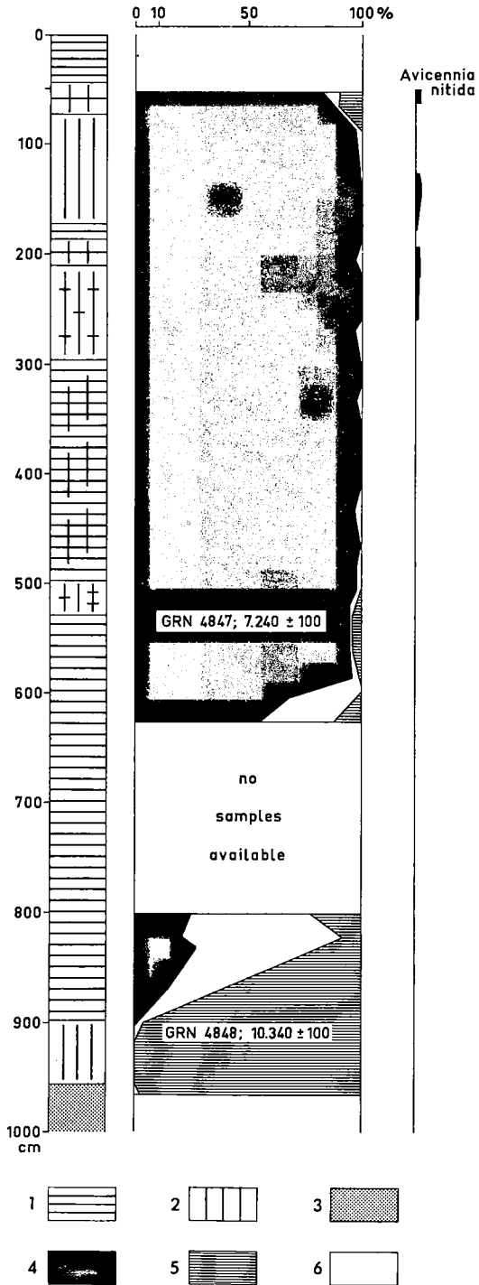
Fig. 6 *. Pollen-analytical profile Matararibo
