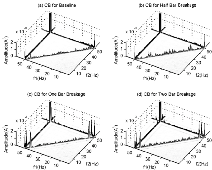
Figure 6. CB amplitudes for baseline motor and BRB cases.
