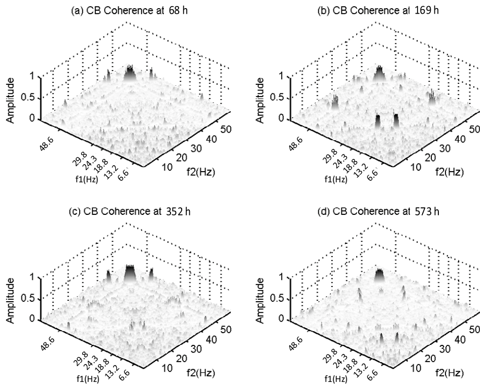
Figure 11. CB coherences for gearbox at successive time instants.
