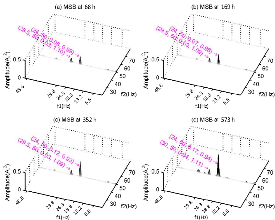
Figure 8. MSB amplitudes for gearbox deterioration at successive time instants.
