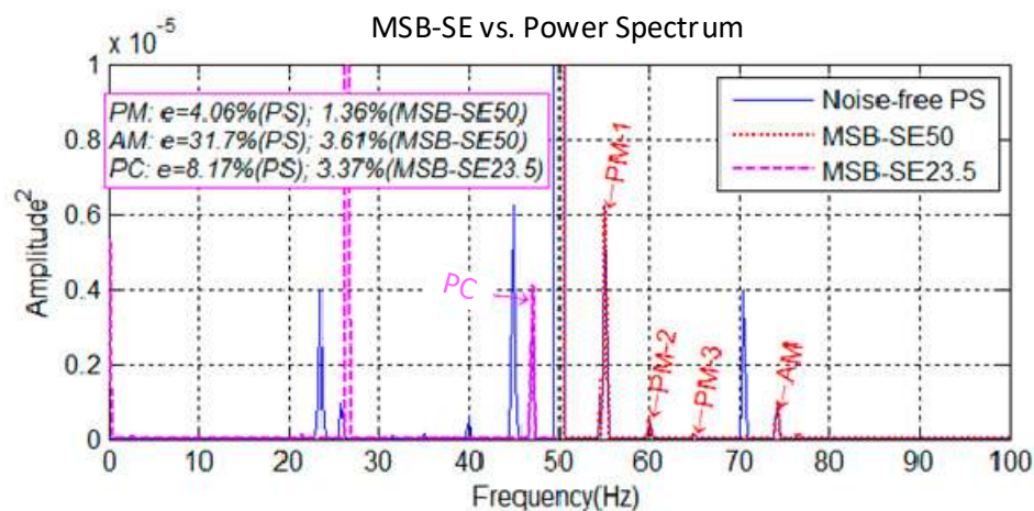
Figure 3. Performance of MSB estimator.
