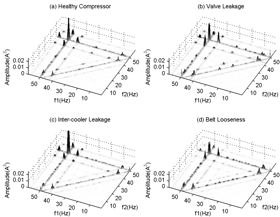
Figure 14. CB coherences for different conditions of the reciprocating compressor.
