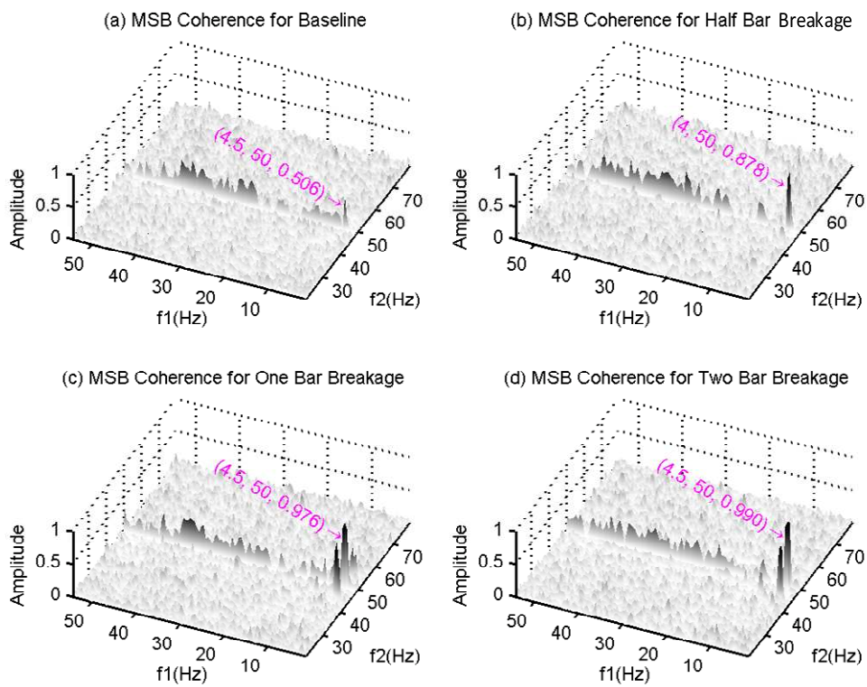
Figure 5. MSB coherences for baseline motor and BRB cases.
