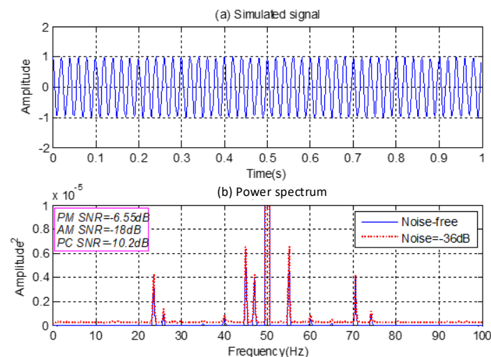
Figure 1. Simulated signals (a) and their power spectra (b).
