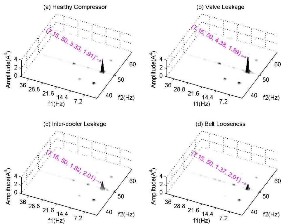
Figure 12. MSB amplitudes for different conditions of the reciprocating compressor.
