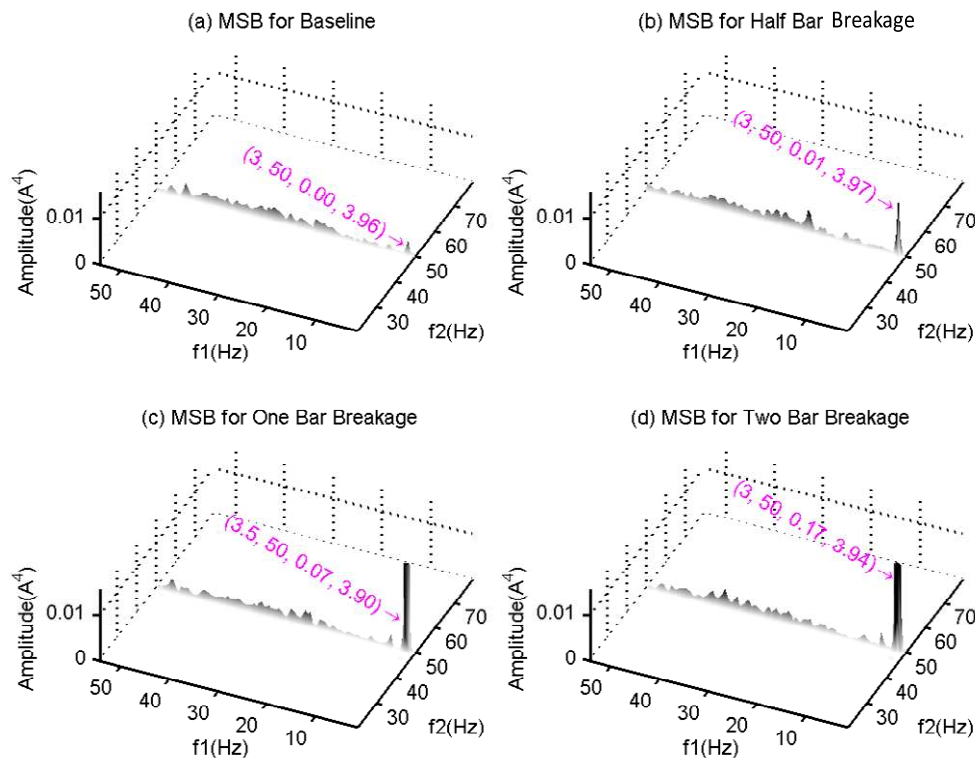
Figure 4. MSB magnitudes for baseline motor and BRB cases.
