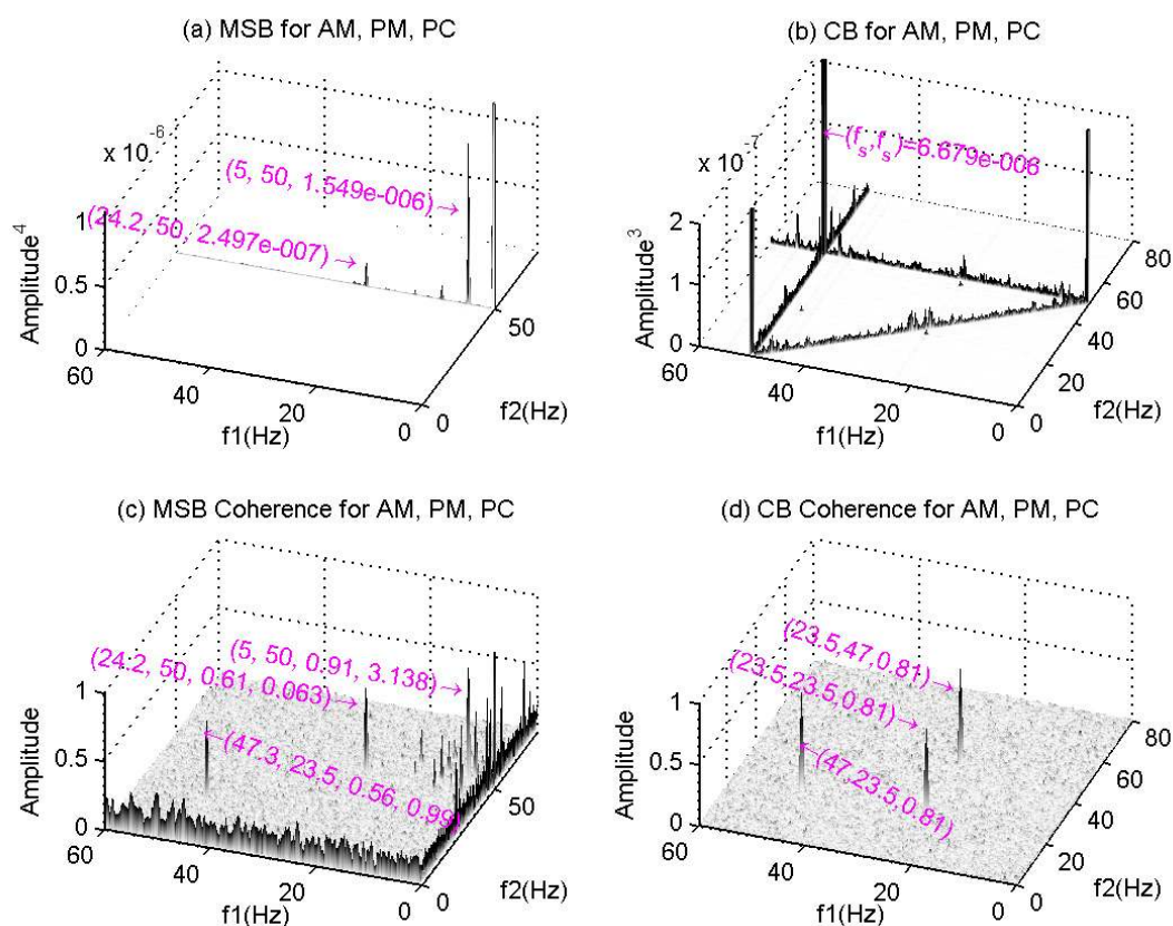
Figure 2. MSB and CB of simulated signal.
