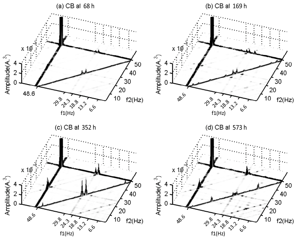
Figure 10. CB amplitudes for gearbox deterioration at successive time instants.
