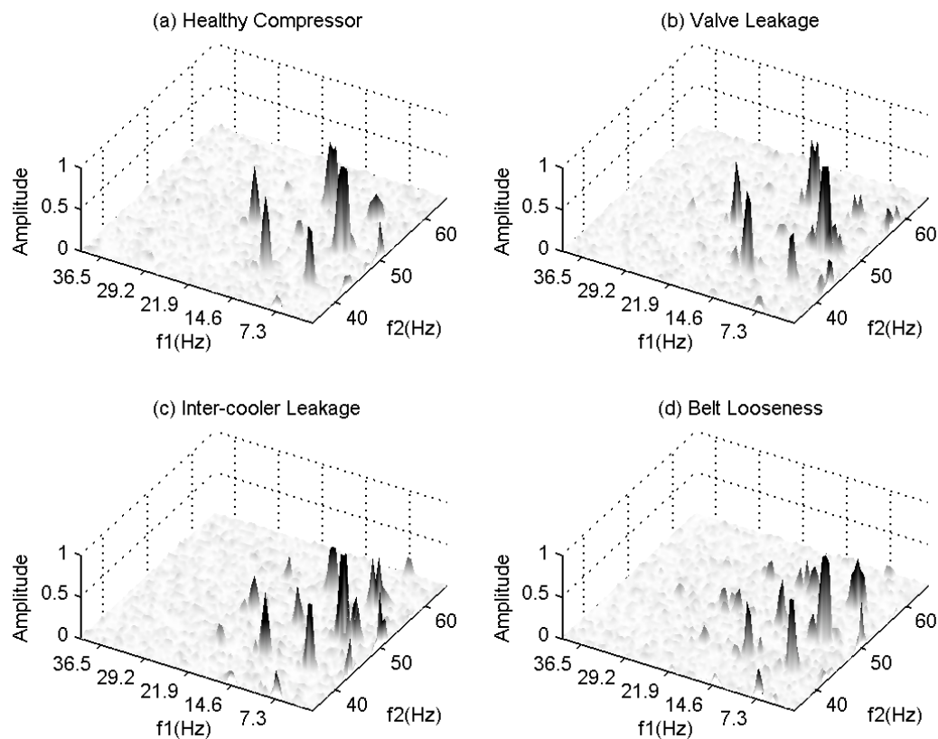
Figure 13. MSB coherences for different conditions of the reciprocating compressor.
