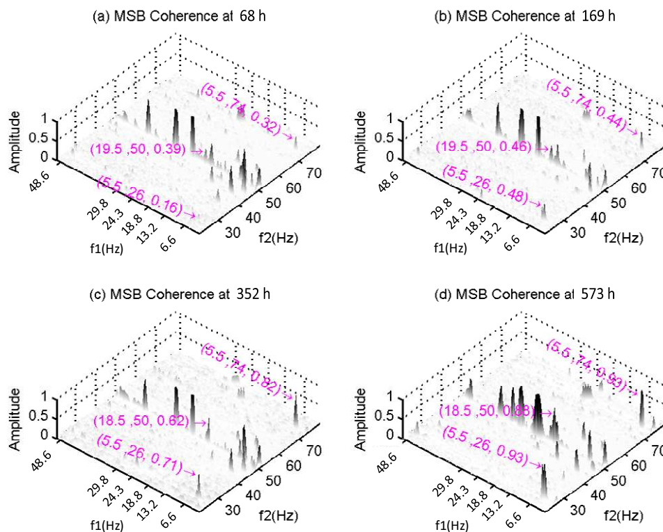
Figure 9. MSB coherences for gearbox deterioration at successive time instants.
