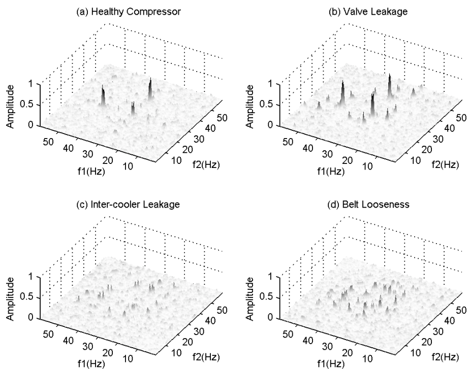
Figure 15. CB coherences for different conditions of the reciprocating compressor.
