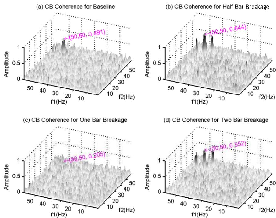
Figure 7. CB coherences for baseline motor and BRB cases.
