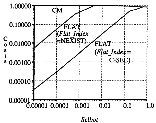
Figure 10: Effect of Flat_Index on FLAT (Query Type 2, PROC_MIX = 0.0001)
