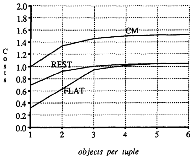
Figure 9: Effect of objects_per_tuple (Query Type 2, PROC_MIX = 0.0001)
