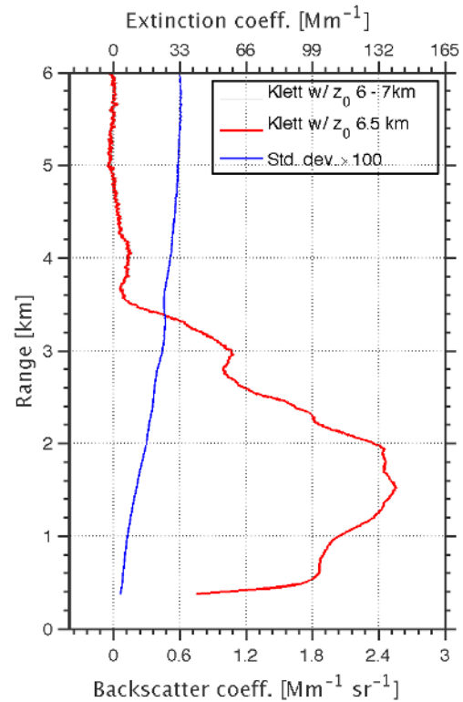
Figure 8. Backscatter coefficient obtained with the Klett algorithm with reference height z_0 varying from 6 to 7 km in steps of 50 m (gray) and the default inversion with z_0 = 6.5 km (red) are shown. The standard deviation shown in blue was multiplied by 100. Data from 1 September 06:30 p.m. to 2 September 05:00 a.m. was used. The extinction scale on top was scaled with L_p = 55 sr.
