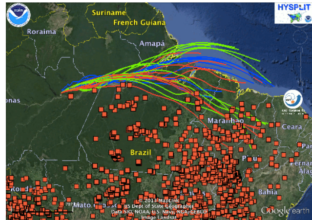
Figure 17. Back trajectories from the Hysplit model from NOAA and fire spots from Instituto Nacional de Pesquisa Espaciais (INPE)'s fire detection algorithm are shown over a Landsat image of the region obtained with Google Earth. Hysplit was run in ensemble mode, with trajectories starting from 1.5 km on 12:00 UTC 3 September. All fire spots from 30 August to 1 September are shown.
