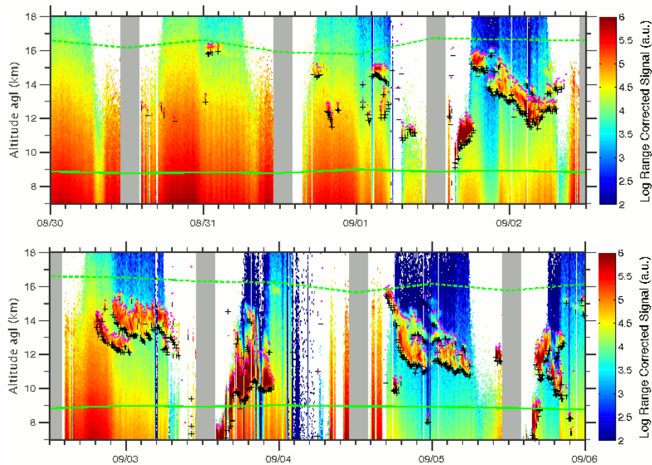
Figure 18. Logarithm of range corrected signal above 7 km is shown from 30 August to 6 September 2011 divided into two panels for depicting the high clouds. Cloud base (+, black) and top (o, magenta) detected by our algorithm are indicated with markers. Full and dashed green lines indicate the -25^{\circ}\text{C} and tropopause heights calculated from the radiosondes. Gray regions correspond to local solar.
