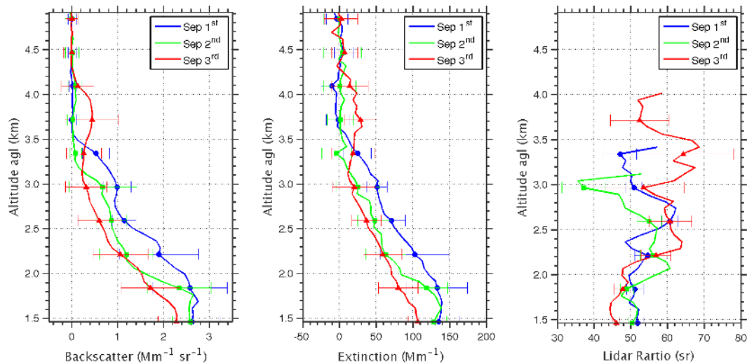
Figure 12. Average aerosol backscatter (left, \text{Mm}^{-1} \text{sr}^{-1} ), extinction (middle, \text{Mm}^{-1} ) and particle lidar ratio (right, sr) obtained from a Raman inversion are shown for days 1, 2 and 3 September 2011.
