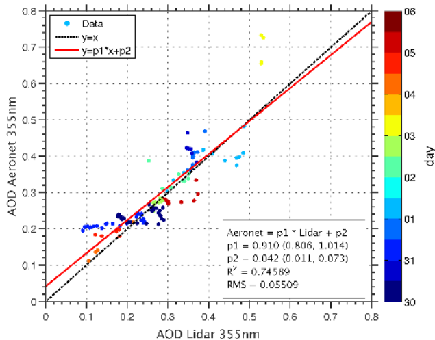
Figure 16. Aerosol optical depth at 355 nm from AERONET as a function of that obtained from the elastic inversion is shown for the coincident measurements between 30 and 6 September 2011. Lidar extinction profiles were averaged in a 30 min window and integrated from the reference altitude down to the ground, assuming a constant extinction below 1.3 km.
