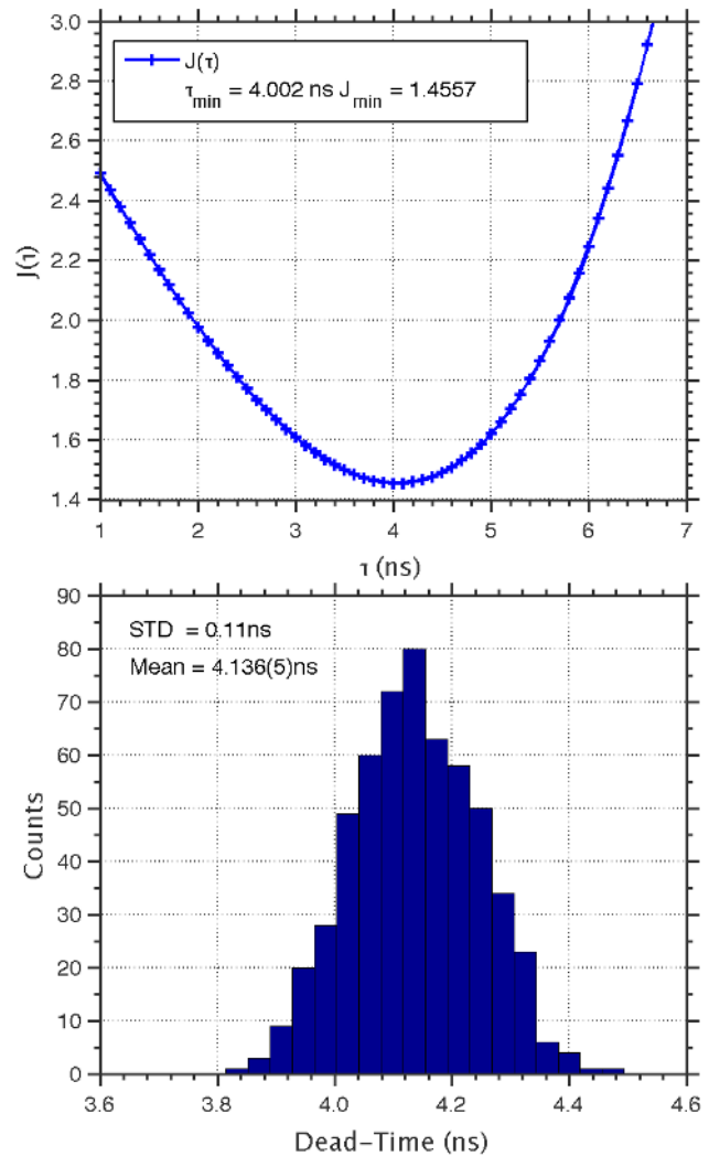
Figure 2. Residual, J(t, \tau) , as a function of the dead time, \tau , for a sample 1 min profile for the elastic channel is shown on top. The point of minimum indicated in the legend is found by fitting a parabola. The lower panel shows the histogram of the dead times for the same channel obtained from 580 independent 1 min profiles. The average and standard deviation are indicated.
