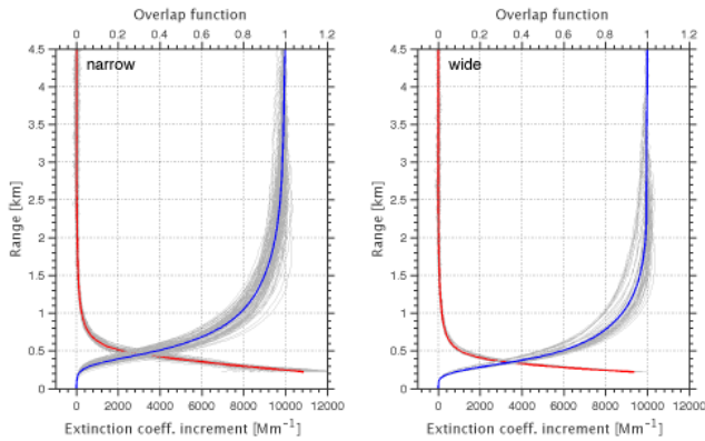
Figure 5. Mean overlap function from 90 (45) cloud and fog free nighttime one-hour profiles measured with a narrow (wide) field stop is shown in blue on the left (right) panel. Mean contribution to the extinction coefficient, as computed from Eq. (14), is shown in red. The gray lines correspond to the individual profiles. The wide field stop is used since 1 August 2012.
