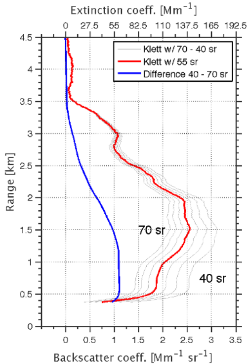
Figure 9. Backscatter coefficient obtained with the Klett algorithm using particle lidar ratios from 40 to 70 sr in steps of 5 sr (gray) and the default inversion with 55 sr (red) are shown. The difference of the backscatter obtained with 40 and 70 sr (blue) is shown as an indication of the uncertainty. Data from 1 September 06:30 p.m. to 2 September 05:00 a.m. was used. The extinction scale on top was scaled with L_p = 55 sr.
