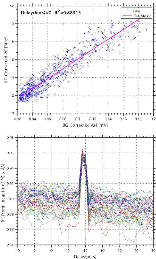
Figure 1. Sample fitting between the PC and channel in the linear region (top) and lag-correlation as a function of the lag for all profiles in one-hour of measurements (bottom) are shown.
