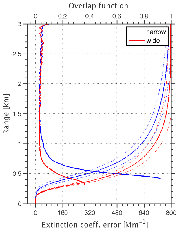
Figure 7. Estimation of the error in the extinction coefficient from the uncertainty in the overlap function are shown in thick lines. For reference, the mean overlap functions and the 95 % confidence level are to the right. Red (blue) colors are used for the wide (narrow) the field stops.
