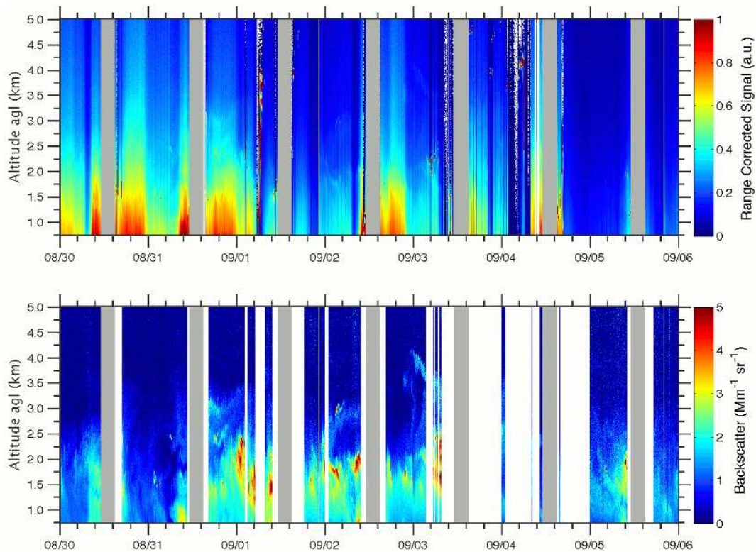
Figure 10. Range and background corrected signal (top, a.u.) and aerosol backscatter coefficient (bottom, \text{Mm}^{-1} \text{sr}^{-1} ) obtained from the elastic channels are shown below 5 km from 30 August to 6 September 2011. Inversion assumed a particle lidar ratio of 55 \text{sr}^{-1} . Gray and white regions correspond to local solar noon and clouds, respectively.
