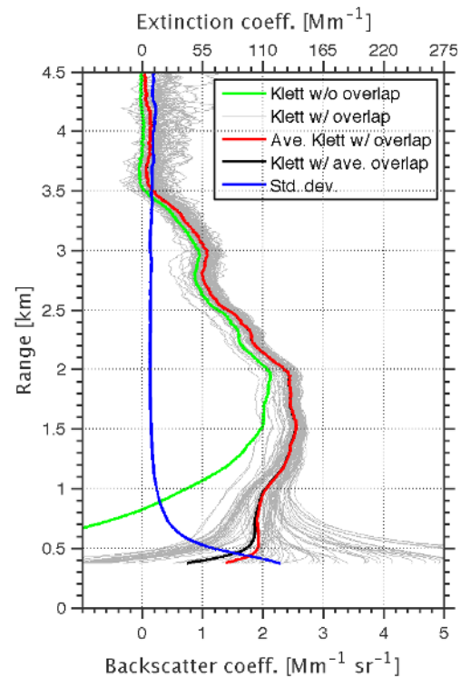
Figure 6. Backscatter coefficient obtained with the Klett algorithm without overlap correction (green) and with the average overlap (black) are shown. The backscatter coefficient obtained for each of the 90 overlaps measured with a narrow field stop (gray), their average (red) and standard deviation (blue) are also shown. Data from 1 September 06:30 p.m. to 2 September 05:00 a.m. was used. The extinction scale on top was scaled with L_p = 55 sr.
