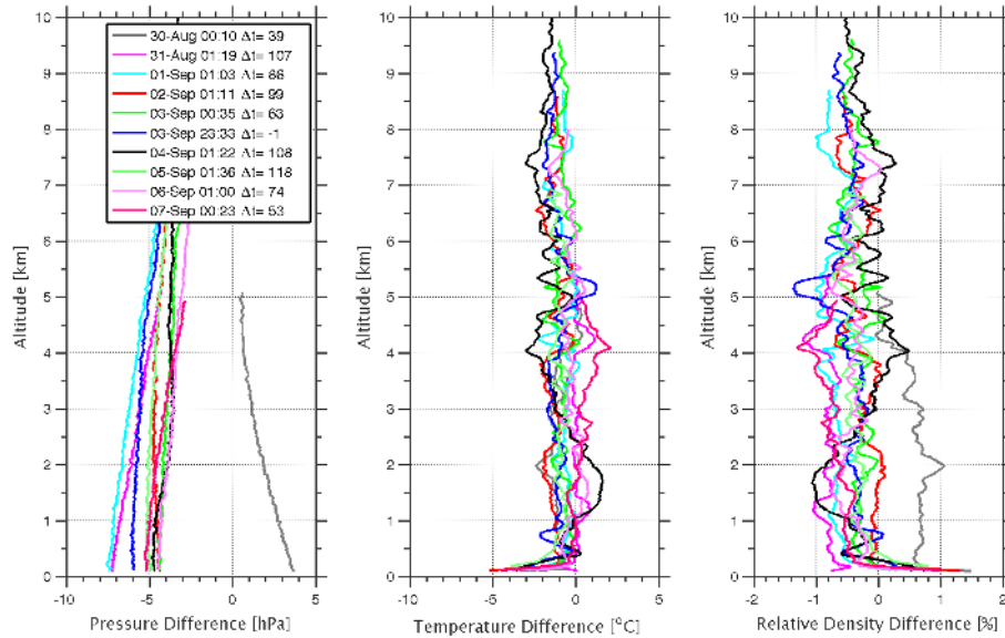
Figure 4. Pressure (hPa, left), temperature ( ^{\circ}\text{C} , center) and relative air density (% , right) differences between the Embrapa's and operational's radiosondes are shown. Dates in the legend correspond to the launching time at the lidar site.
