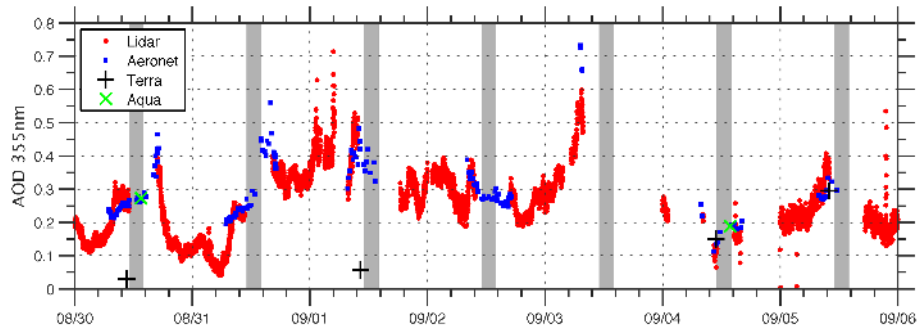
Figure 14. The time series of aerosol optical depth at 355 nm obtained from the elastic inversion (red), AERONET (blue), MODIS-Terra (black) and MODIS-Aqua (green) are shown between 30 August and 6 September 2011. Gray regions correspond to local solar noon.
