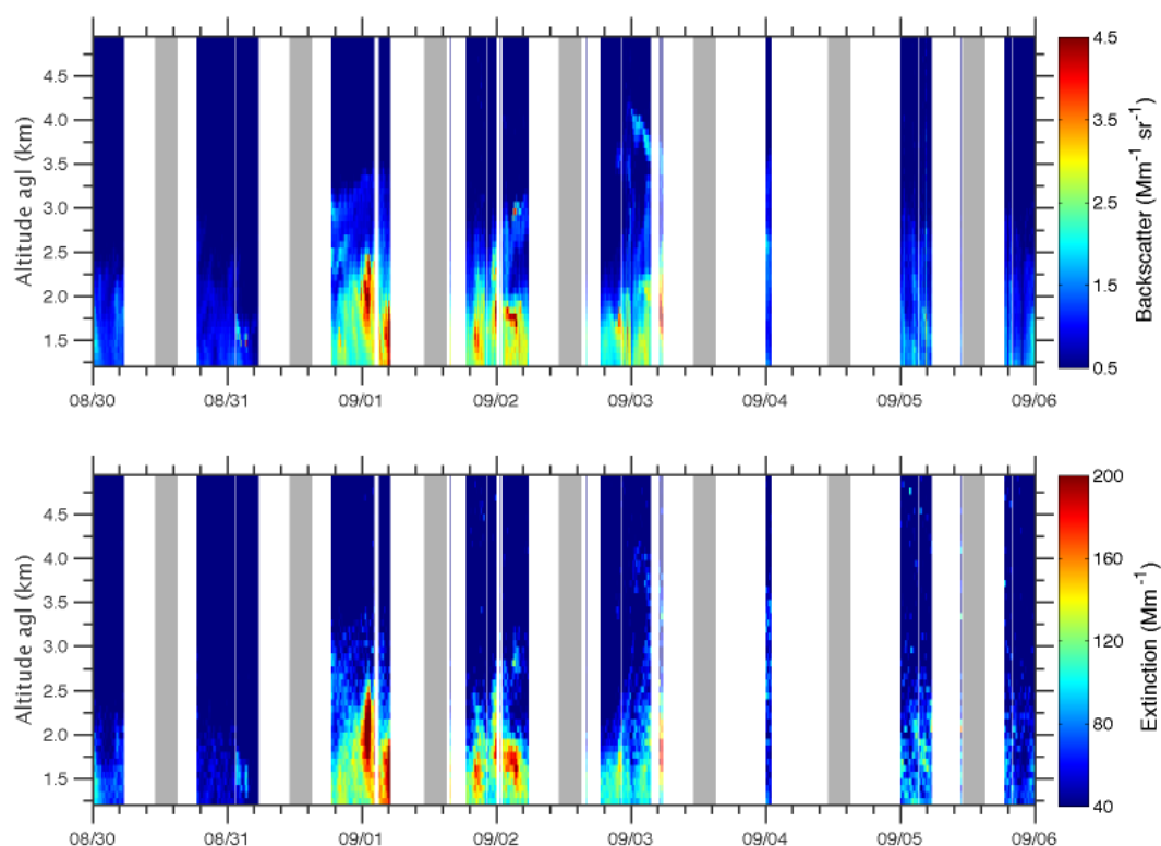
Figure 11. Aerosol backscatter (top, \text{Mm}^{-1} \text{sr}^{-1} ) and extinction (bottom, \text{Mm}^{-1} ) obtained from a Raman inversion are shown above 1 km from 30 August to 6 September 2011. Gray and white regions correspond to local solar noon and clouds, respectively.
