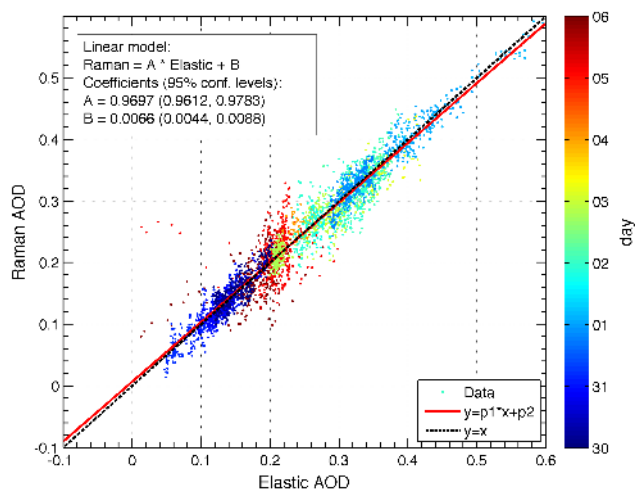
Figure 13. Aerosol optical depth at 355 nm obtained from the Raman inversion is shown as a function of the optical depth from the elastic inversion for 4435 nighttime cloud-free 1 min profiles between 30 August and 6 September 2011. Colors indicate day of month. The two lines are the linear regression (continuous red) and the reference y = x (dashed).
