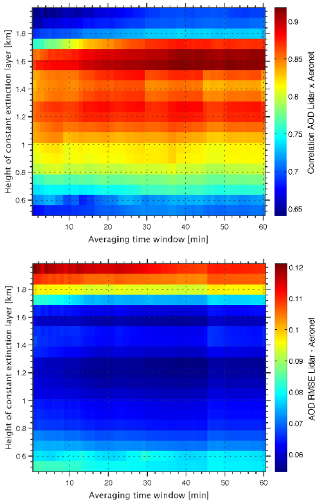
Figure 15. Time correlation (top) and root mean square error (RMSE, bottom) between AERONET AOD and elastic lidar AOD time series are shown as a function of the averaging time window and the height of the constant extinction layer.
