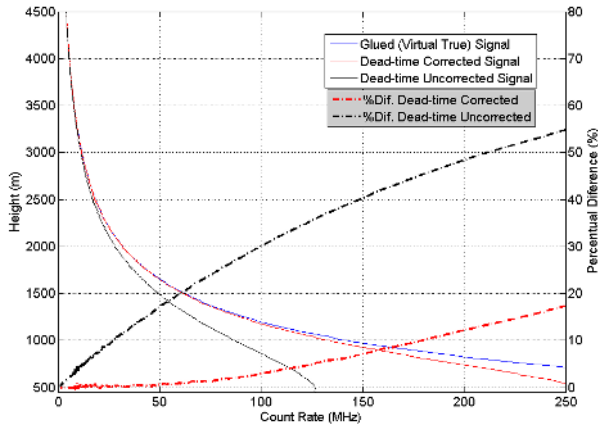
Figure 3. Corrected (thin red) and uncorrected (thin black) count rates (MHz) from a sample 20 min profile from the elastic channel are shown. The difference (%) between these and the true count rate (glued, thin blue) is given by the red and black dot-dashed lines, respectively.
