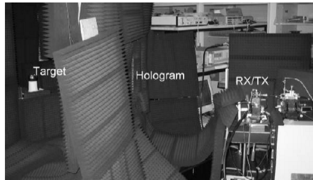
Figure 3. Test RCS measurement facility.
