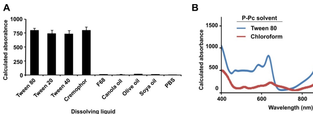
Figure 2. Absorbance of P-Pc in excipients. (A) Calculated absorbance of P-Pc at 997 nm following dissolution in the indicated liquids at 20 mg/mL P-Pc. Samples were briefly centrifuged prior to measurement in a cuvette with a 10 \mu\text{m} path length. Absorbance was multiplied by 1000 to produce calculated absorbance based on a 1 cm path length (mean \pm s.d. for n = 3 ). (B) Calculated absorbance of 40 mg/mL P-Pc dye in Tween 80 (blue) or 20 mg/mL in chloroform (red). The Tween formulation was measured directly with a 10 \mu\text{m} path length cuvette. Since chloroform was not compatible with the 10 \mu\text{m} path length cuvette, it was diluted 1000 times into a conventional cuvette. Absorbance was multiplied by 1000 for calculated absorbance of the solution, based on a 1 cm path length.
