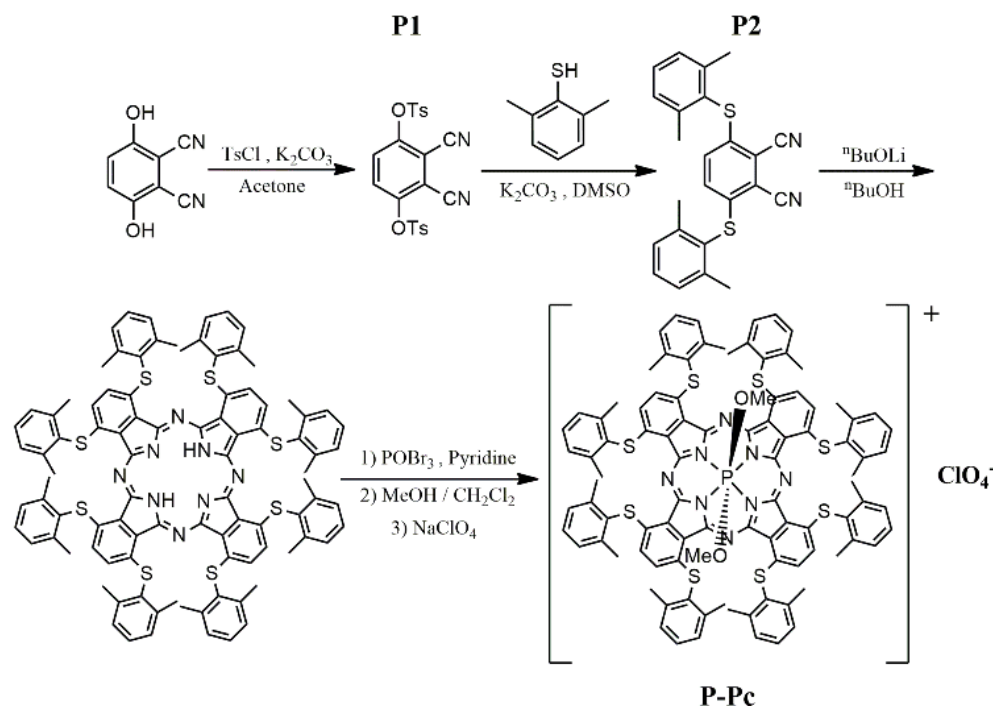
Figure 1. Synthesis of phosphorus phthalocyanine (P-Pc): [\alpha\text{-(2,6-dimethylphenylthio)}_6\text{PcP(OMe)}_2]^+[\text{ClO}_4]^-
