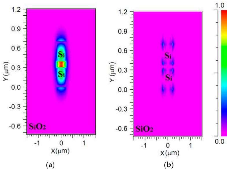
Figure 3. Quasi-transverse magnetic (TM) fundamental field profile mode for the 1 \times 4 power splitter: (a) Major mode E_y ; (b) minor mode E_x .
