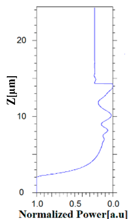
Figure 6. Propagation distance Z as a function of power propagation.
