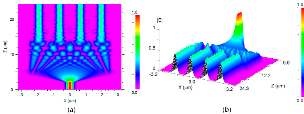
Figure 5. The propagation profile of the electric field for the 1 \times 4 MMI power splitter at x - z plane: (a) 2D; (b) 3D.
