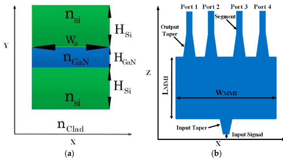
Figure 1. Schematic illustration of the optical 1 \times 4 power splitter: (a) x – y plane; (b) x – z plane.
