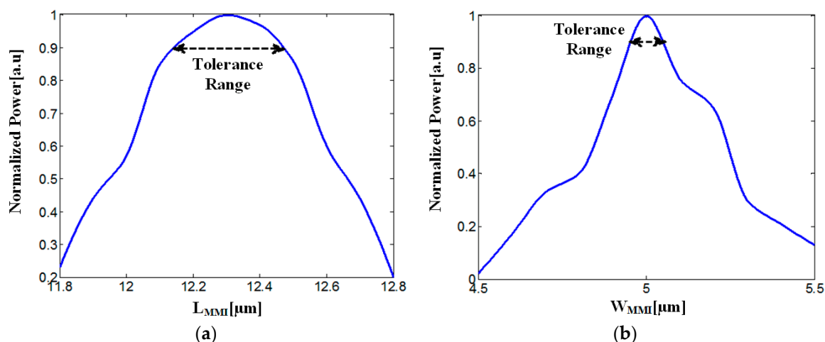
Figure 4. Normalized power as function of the geometrical multimode interference (MMI) coupler parameters: (a) L_{\text{MMI}} ; (b) W_{\text{MMI}} .
