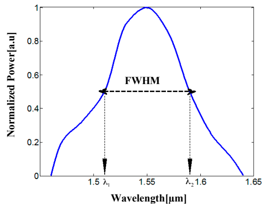
Figure 7. Normalized power as function of wavelength.
