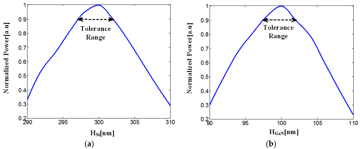
Figure 2. Normalized power at the slot area as a function of the geometrical parameters: (a) H_{Si} ; (b) H_{GaN} .
