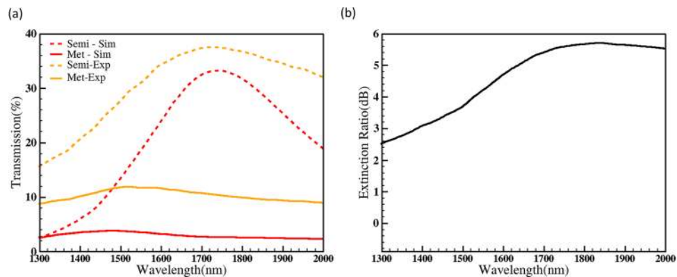
Figure 6. (a) Transmission spectra of the photonic switch (570 nm diameter and 1010 nm pitch) for the aluminium thickness of 80 nm, 20 nm Cr and 25 nm \text{VO}_2 for semiconductor phase (dash line) and metallic phases (solid line) from experiments and simulations. (b) The extinction ratio of the switch measured from experiments (Extinction ratio: 4.3 dB in C-band, 4.9 dB in L-band and 5.3 in U-band).
