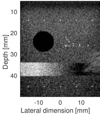
Fig. 4. Log-compressed B-mode image of the PICMUS numerical phantom.
