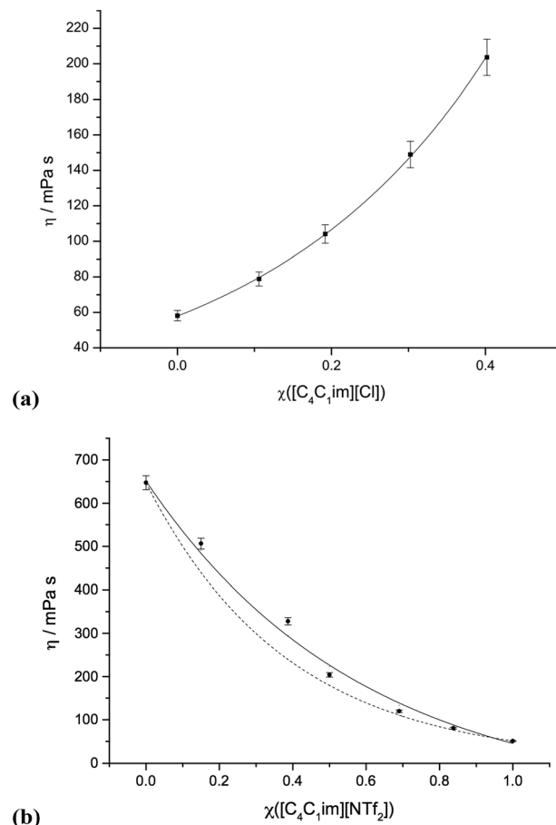
Fig. 5 Viscosities of mixture series: (a) [C_4C_1im][Cl][OTf] , 1 ; (b) [C_4C_1im][NTf_2][Me_2PO_4] , 7 . The dashed line in (b) represents the ideal Katti and Chaudhri mixing law (eqn (2)), continuous lines include the additional f non-ideality parameter of Grunberg and Nissan (eqn (3)).
