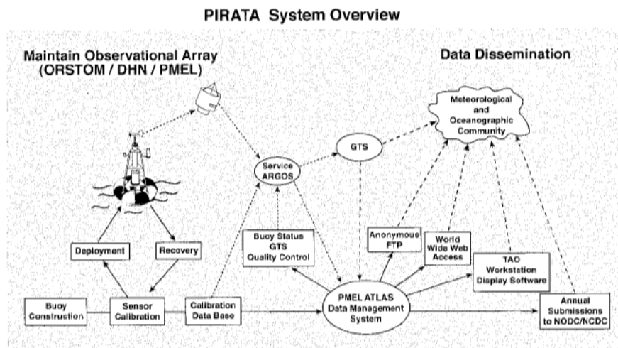
FIG. 7. Schematic of the PIRATA real-time data flow.
