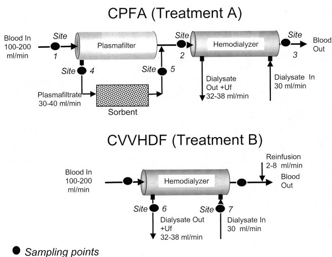
Figure 1. Schematic representation of the two treatment circuits (treatment A: coupled plasma filtration adsorption [CPFA]; treatment B: continuous venovenous hemodiafiltration [CVVHDF] and of the sampling points evaluated in this study. Sampling points 2 and 3 were approximately 10 cm from the plasma reinfusion site and the hemodialyzer, respectively. Uf , ultrafiltration.
