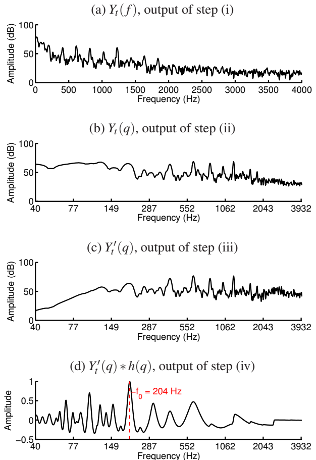
Figure 2: Algorithm processing steps for a single voiced frame of speech corrupted with car noise. (a) PSD in dB, (b) PSD in dB in a log-frequency grid, (c) compressed PSD in dB in a log-frequency grid, and (d) normalized output of the filter and fundamental frequency, f_0 .
