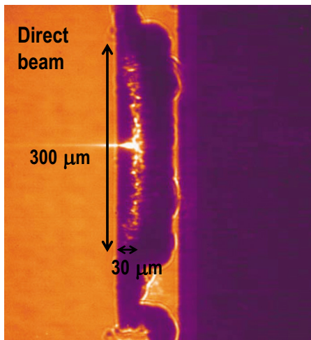
FIG. 4. (Color online) X-ray image of the diamond lens structure. The bright spot in the middle is the microfocused beam. The orange area is the unfocused monochromatic incident x-ray beam. The purple areas are the diamond lens structure, easily recognized by looking at the SEMs in Fig. 2, and the diamond carrier chip to which the nanocrystalline diamond was glued before the silicon etch.
