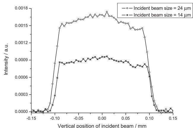
FIG. 7. Pencil beam scan of the lens aperture. The data are the integrated flux in the focal spot vs pencil-beam position for incident vertical beam sizes as indicated in the legend.
