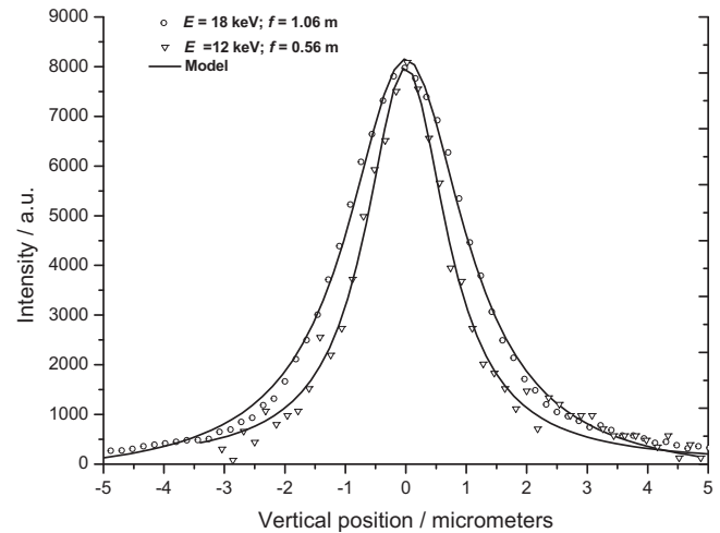
FIG. 5. Vertically focused beam profiles extracted from a detector image. The data are the results from two different experiments, at different values of the energy and of the focal length as summarized in Table I. Two different lenses on the same chips were used. The model (solid line) is a Lorentzian curve that fits the data and provides the following values for the focused beam FWHM: 2.2 \mu\text{m} (open circles) and 1.6 \mu\text{m} (triangle) as reported in Table I.
