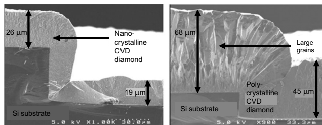
FIG. 2. SEM images of sliced diamond layers deposited on silicon molds. These images illustrate the different quality of diamond material achieved with different deposition chemistry. Left: nanocrystalline diamond, believed to provide better lenses due to reduced unwanted scattering, and used for experiment described in this paper. Right: microcrystalline diamond unsuitable for synchrotron optics.
