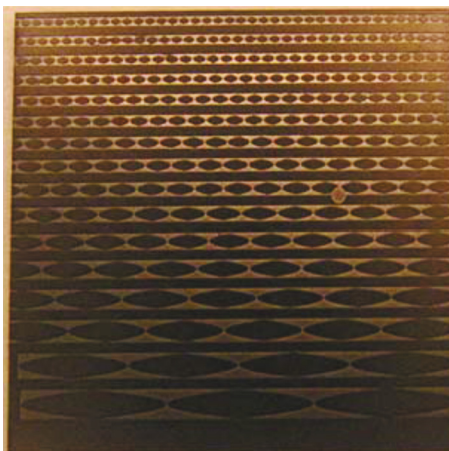
FIG. 1. (Color online) Optical microscope image of a silicon template chip with diamond deposited on top. The chip dimensions are 20 mm \times 20 mm.
