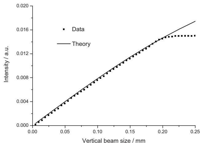
FIG. 6. Intensity of the focal spot as a function of size of the incident beam, with E=18 keV, and f=1.06 m. The theoretical values are the product of three factors: theoretical transmission; beam size; arbitrary scaling factor. The experimental data are the integrated flux in the focal spot.
