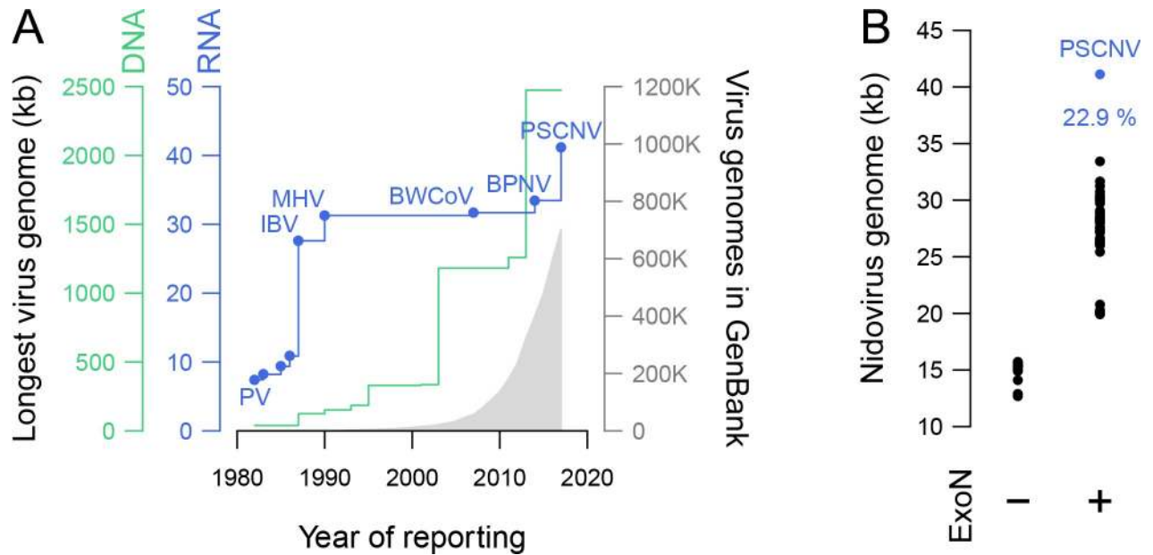
Fig 1. Genome sizes of nidoviruses. (A) Timeline of discovery of largest RNA and DNA virus genomes versus accumulation of virus genome sequences in GenBank (1982–2017). PV, poliovirus; and nidoviruses: IBV, avian infectious bronchitis virus, MHV, mouse hepatitis virus, BWCoV, beluga whale coronavirus SW1, BPNV, ball python nidovirus and PSCNV, planarian secretory cell nidovirus. (B) Comparison of genome sizes between nidoviruses that do not encode an ExoN domain, and those that do. Percentage indicates the difference between sizes of PSCNV and the next-largest entity.
