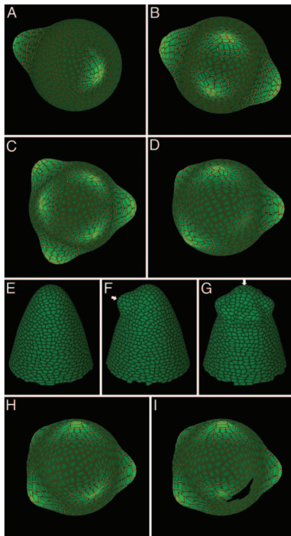
Fig. 4. Simulated shoot apical meristems. (A–D) The arrangement of primordia into phyllotactic patterns: distichous (A), decussate (B), tricusate (C), and spiral (D). (E–G) Simulated pin1 mutant (E), primordium formed in the pin1 mutant after localized application of auxin in the peripheral zone (F), and primordium ring formed in the pin1 mutant after localized application of auxin at the tip of the apex (G). Arrows indicate the site of auxin application. (H and I) Simulated results of cell ablation: control apex (H) and the apex in which five cells shown in black have been removed (I). Note the shift in the position of the primordium initial (cells with high auxin concentration, shown in bright green) near the ablation site.
