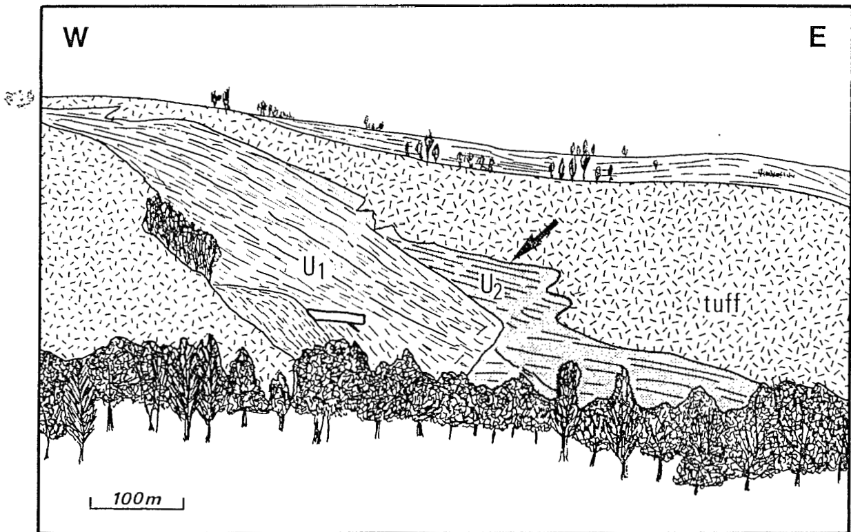
Figure 8. Illustration of the onlap wedges (arrow) on the eastern limb of Jachahuanguo fold.
