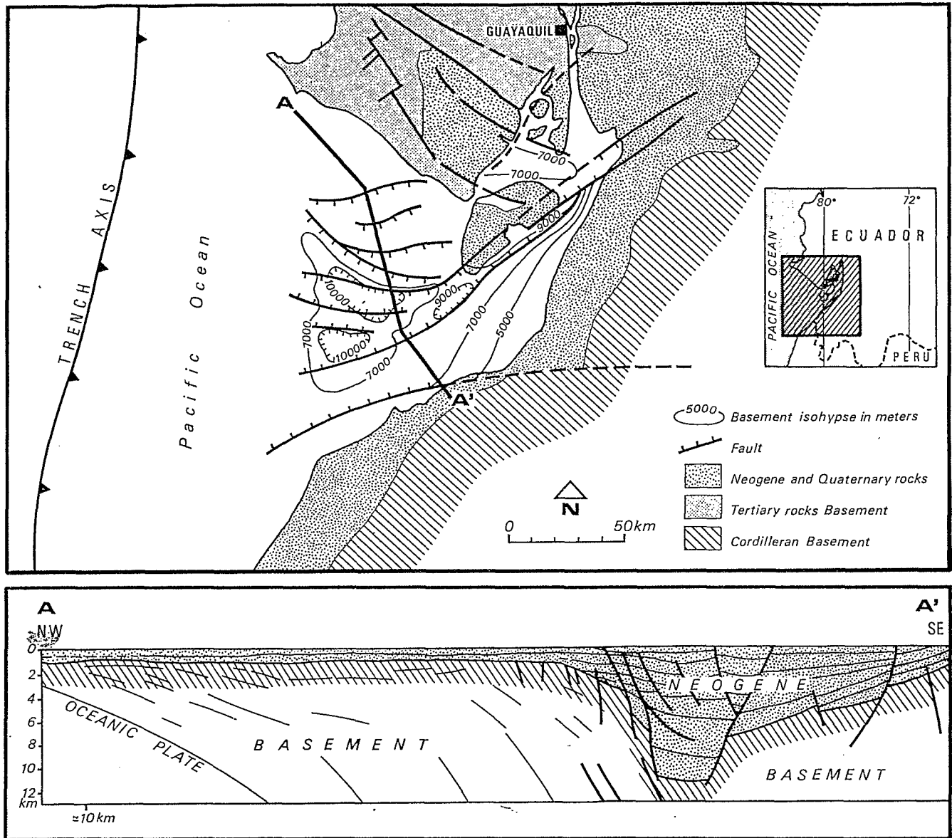
Figure 16. Simplified geological sketch map of the Gulf of Guayaquil and NW-SE cross-sections through the Jambeli channel showing the 10 000 m thickness of Neogene deposits (modified after Benitez 1986).
