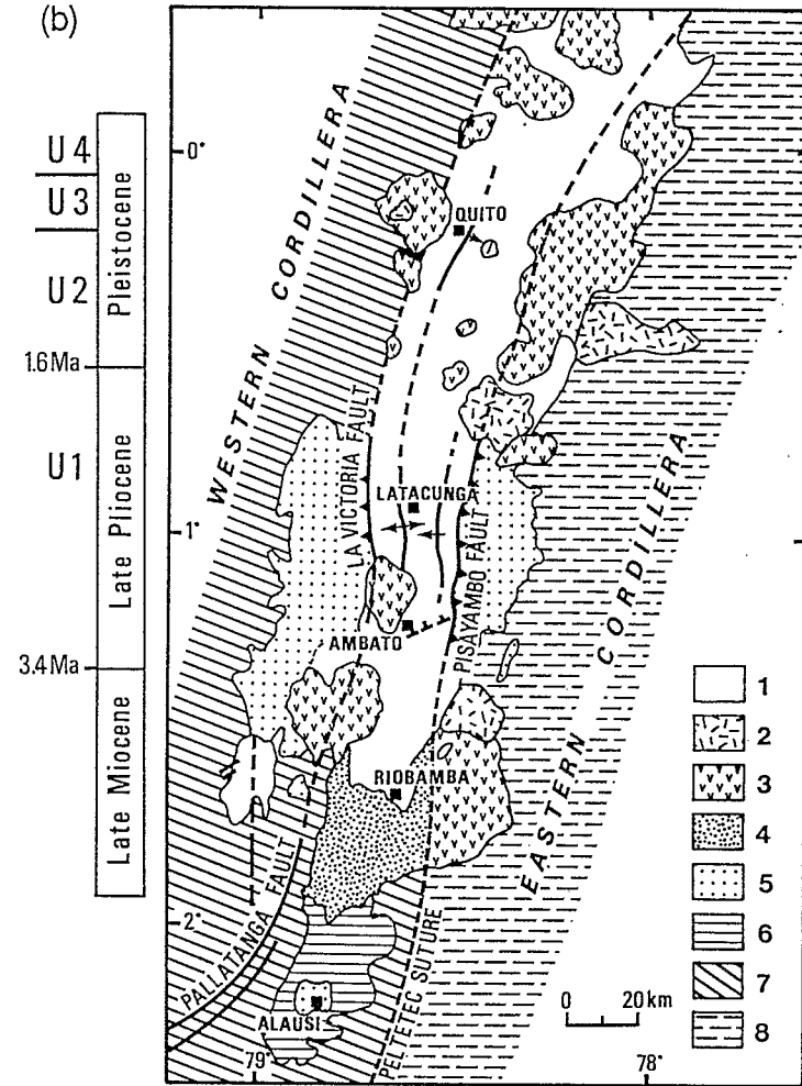
Figure 3. (a) Synthetic stratigraphic sections from the Western Cordillera (A) and Interandean Depression (B) in Central Ecuador: radiometric dates from Barberi et al. (1988) and Lavenu et al. (1992). (b) Schematic geological map of the south Interandean Depression (after DGGM 1982, modified). 1: Quaternary deposits; 2: Quaternary volcanic rocks; 3: Pliocene volcanic rocks; 4: Pliocene sedimentary rocks; 5: Miocene sedimentary and volcanic rocks; 6: Oligocene rocks; 7: Western Cordillera; 8: Eastern Cordillera.
