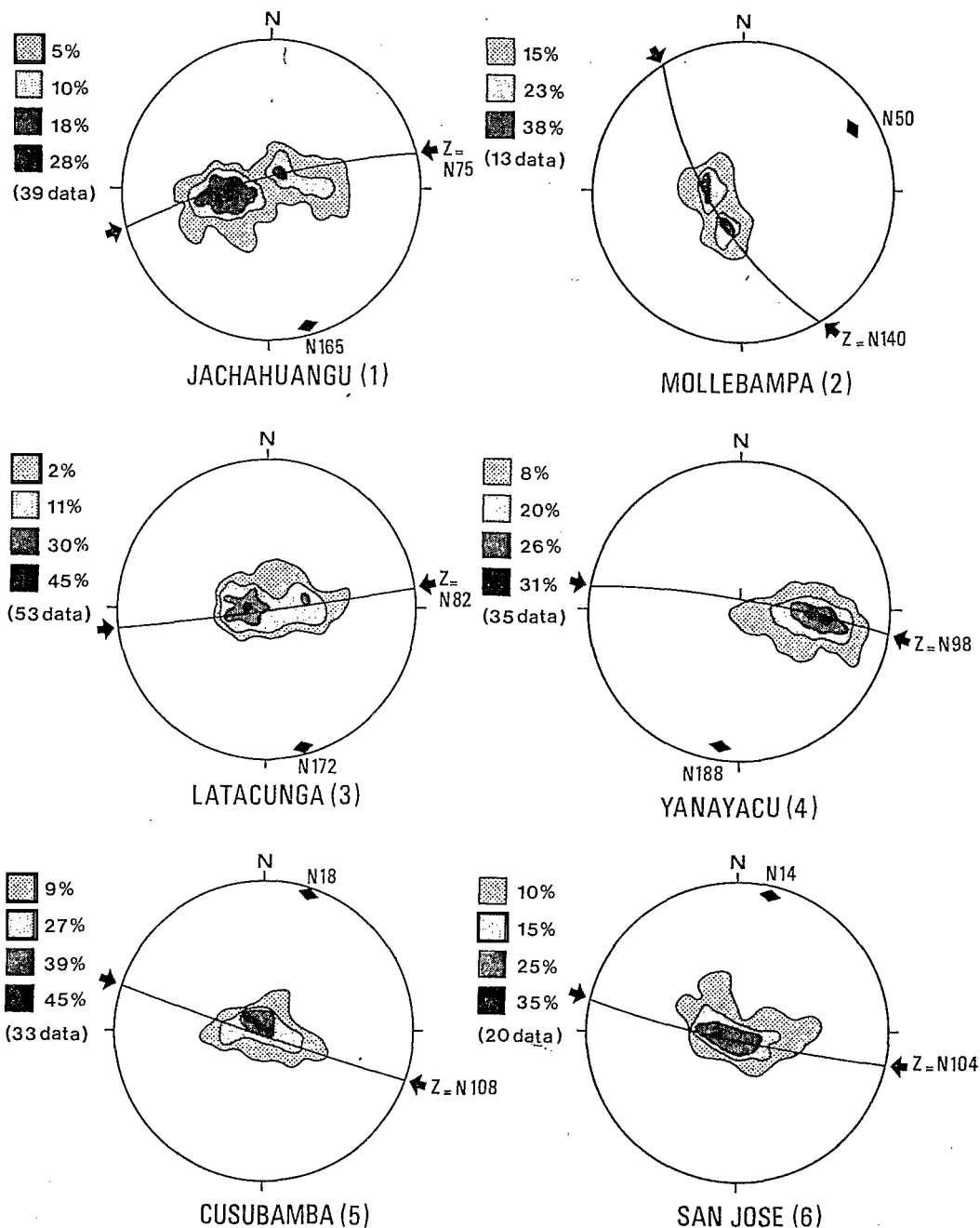
Figure 7. Equal-area stereographic projections depicting poles to bedding in Latacunga zone (lower hemisphere). Contour lines enclose areas of like density of occupation. All the syndimentary folds and flexures (location, Fig. 4) characterize the E-W Pliocene-Quaternary shortening.
