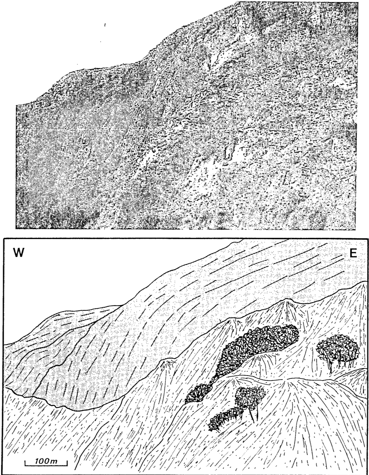
Figure 9. Illustration of the Yanayacu flexure near Bellavista.
