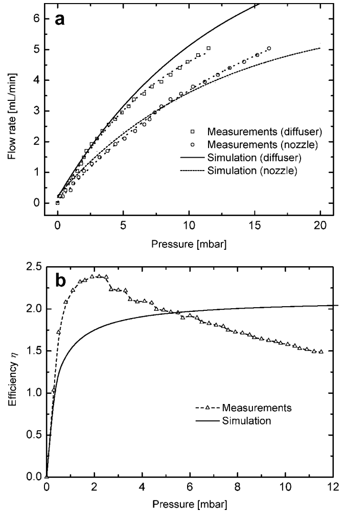
Fig. 9 a Flow rate–pressure measurement for a discrete nozzle/diffuser element, identical to that used in the micropump, but with a thickness of 0.5 mm. b Plot of the efficiency vs. pressure calculated from the results of Fig. 9a using Eq. 5
