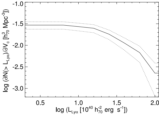
FIG. 9.—Comoving density of emitters with a luminosity exceeding L_{\text{Ly}\alpha} .
