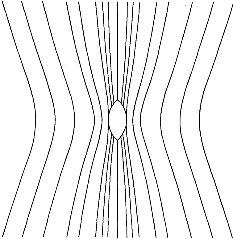
FIGURE 6. The streamlines \psi/c^2U in the laboratory frame for an inert translating prolate spheroid of eccentricity 0.9. Here V_n/U = V_s/U = 0 .
