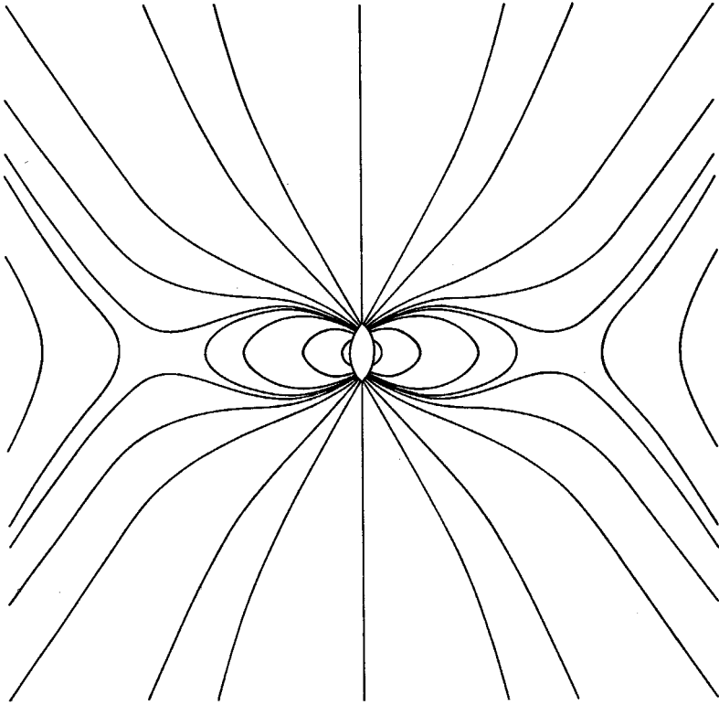
FIGURE 7. The streamlines \psi/c^2U in the laboratory frame for a prolate spheroid having eccentricity 0.9 for the case V_n/U = 0 , V_s/U = 1.17 .
