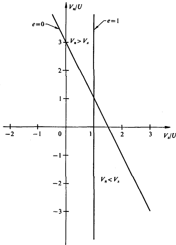
FIGURE 3. The relationship between V_n/U and V_s/U for self-propulsion.
