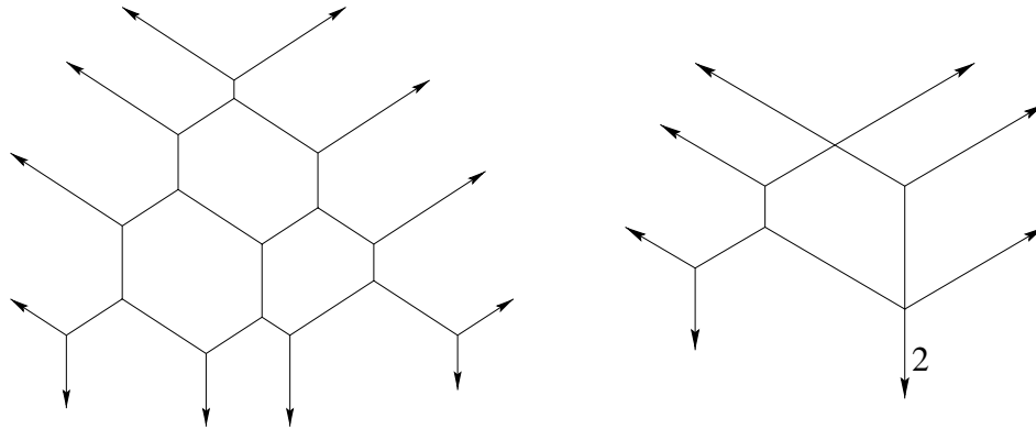
Figure 3: Two honeycombs, of sizes 4 and 3. The left one is more typical in having only \mathbf{Y} vertices. All edges are multiplicity 1, except for the edge labeled 2 in the right-hand honeycomb.
