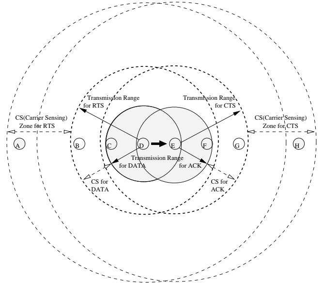
Figure 6: BASIC scheme: Suppose node D transmits a packet to node E. Since DATA and ACK are transmitted using the minimum necessary transmit power, nodes in carrier sensing zone (such as A and H) during the RTS-CTS transmission may not sense any signal during DATA-ACK. When these nodes initiate a new transmission by sending RTS at the power level p_{max} , a collision may occur at D and E. The collisions trigger retransmissions, resulting in more energy consumption.
