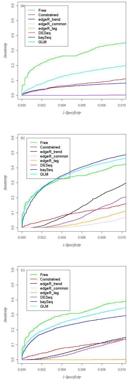
Fig. 3. Portions of ROC curves for Dataset 2. (a) the curve for low-expression genes with the x axis ranging 0-0.01 (see text);(b) a similar set of curves for high-expression genes;(c) all genes, but with a more stringent 1-specificity
