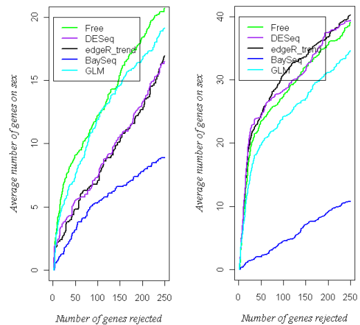
Fig. 4. Number of detected genes on the sex chromosomes vs. number of genes detected, using subsamples from Dataset 3 with n_1 = 6 males vs n_2 = 6 females. (a) the CEU dataset; (b) the YRI data.
