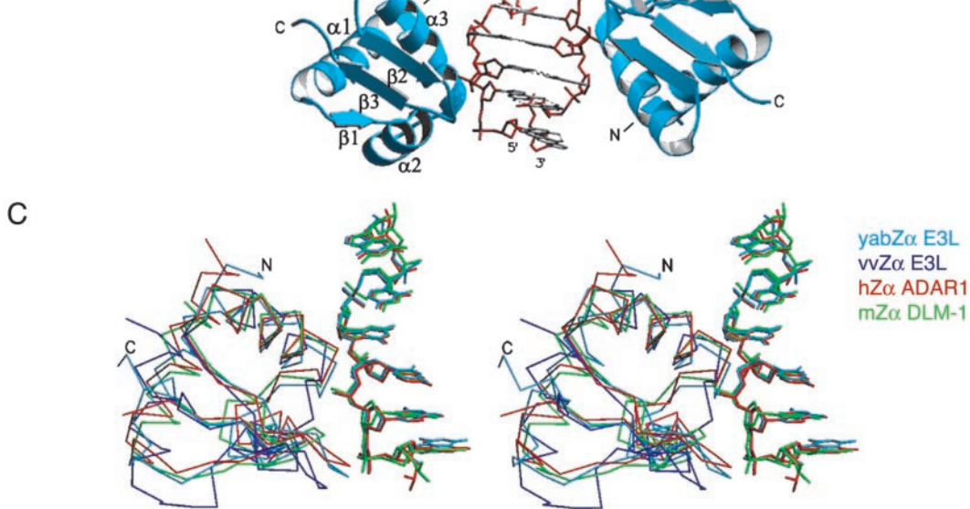
Fig. 1. Sequence and secondary structural comparison of yabZ \alpha_{E3L} with the other Z-DNA-binding domains and related poxvirus E3L domains. (A) Multiple sequence alignment of the Z \alpha proteins. Numbering and secondary structure elements for the Z \alpha domains of E3L from YLDV (yabZ \alpha_{E3L} ), YMTV (ymtvZ \alpha_{E3L} ), vaccinia virus (vvZ \alpha_{E3L} ), Orf virus (ovZ \alpha_{E3L} ), and Swinepox virus (svZ \alpha_{E3L} ), along with human ADAR1 (hZ \alpha_{ADAR1} ) and mouse DLM1 (mZ \alpha_{DLM1} ) (accession numbers as in ref. 16, except YMTV NC 005179). Secondary structure is drawn on top of the sequence. The \alpha -helix and \beta -sheet are represented by tubes and arrows, respectively. The conserved sequences of all Z \alpha family are colored yellow. Residues from yabZ \alpha_{E3L} that make contact with the DNA are marked with a blue triangle. (B) The overall structure of the yabZ \alpha_{E3L} :Z-DNA complex. The N and C terminus and secondary structure elements are labeled. (C) Structural superposition of yabZ \alpha_{E3L} :Z-DNA (sky blue), hZ \alpha_{ADAR1} :Z-DNA (red), mZ \alpha_{DLM1} :Z-DNA (green), and vvZ \alpha_{E3L} (royal blue). All DNA atoms and structurally aligned C \alpha atoms were used for the superposition (64 C \alpha for hZ \alpha_{ADAR1} and 57 C \alpha for Z \alpha_{DLM1} ).
