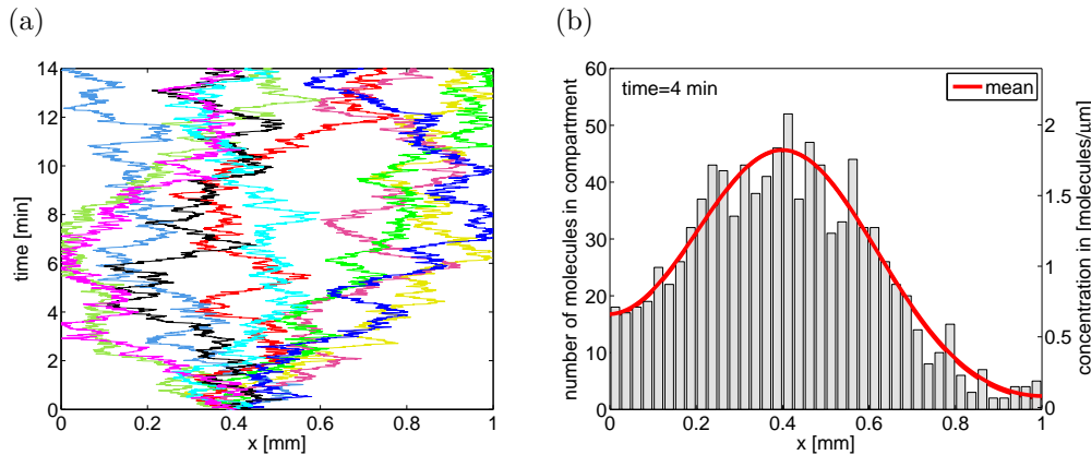
FIG. 3.2. (a) Ten trajectories computed by SSA (a7)–(c7) for D = 10^{-4} \text{ mm}^2 \text{ sec}^{-1} , L = 1 \text{ mm} , X(0) = 0.4 \text{ mm} and \Delta t = 0.1 \text{ sec} . (b) Numbers of molecules in bins of length h = 25 \mu\text{m} at time t = 4 \text{ min} .
