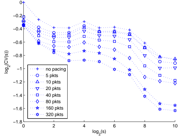
Fig. 9. Pacing effect of QLBP on self-similar Internet traffic
