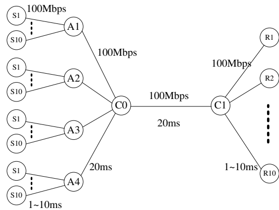
Fig. 10. A dumbbell topology
