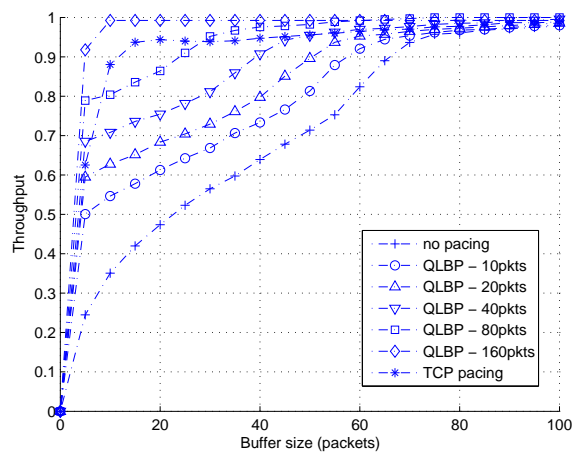
Fig. 11. Link utilization v.s. various buffer size
