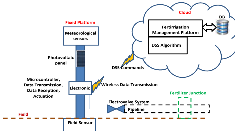
Figure 1. Architecture of the DSS of the project 'DSS Fertirrigation 4th range'.
