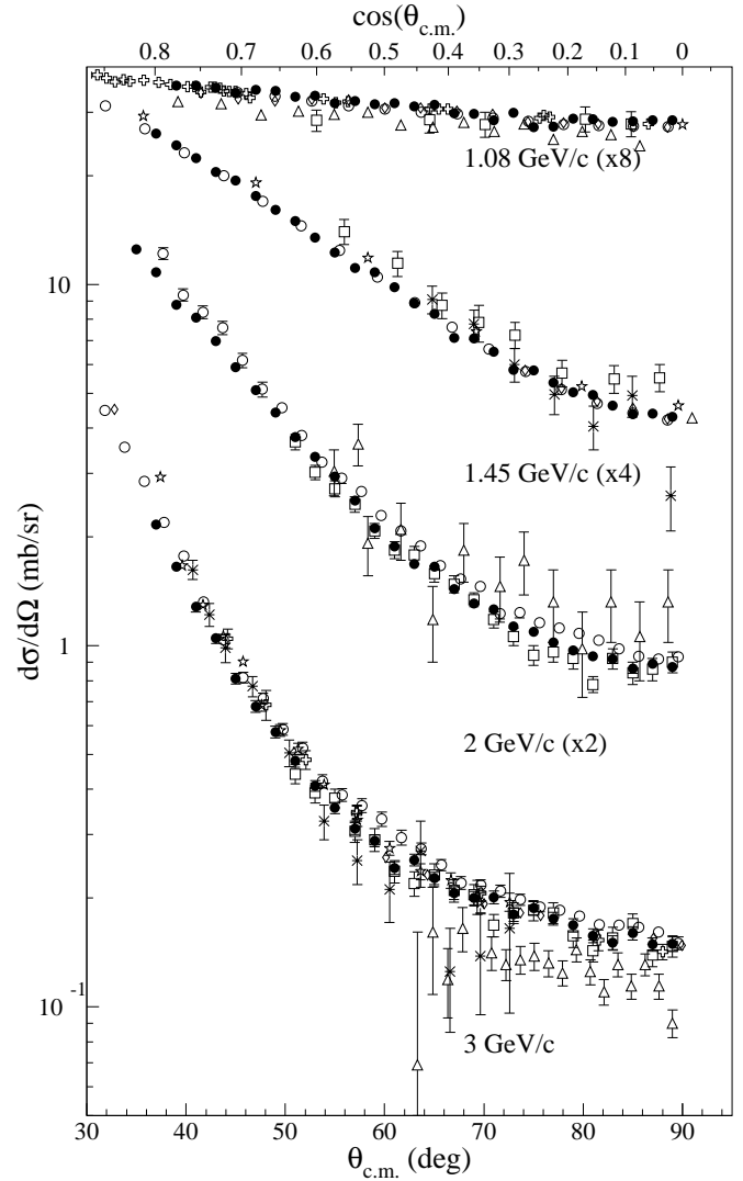
Fig. 26. Angular distributions at four beam momenta. Data of this work ( \bullet ) are compared to published data, where the symbols \circ , \square , \triangle , \diamond , \star , and \times correspond to data from [30, 48, 50, 51, 52, 53] at 1.08 GeV/c, [30, 48, 49, 51, 54, 55, 56] at 1.45 GeV/c, [46, 47, 57] at 2 GeV/c and [45, 46, 47, 58, 59, 60, 61] at 3 GeV/c.
