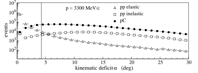
Fig. 9. Simulated distributions of the kinematic deficit \alpha for p-C reactions (solid dots), elastic (triangles) and inelastic (squares) pp scattering. The vertical line indicates the position of \alpha_{cut} .
