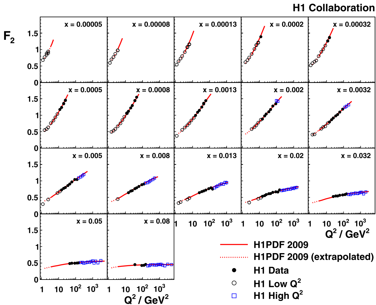
Fig. 6 Measurement of the structure function F_2 as a function of Q^2 at various values of x . The data of this measurement ( closed circles ) are complemented by the previously published data at low Q^2 ( open circles ) [2] and high Q^2 ( open boxes ) [9]. The error bars represent the total measurement uncertainties. The solid curve represents the QCD fit described in this paper for Q^2 \geq 3.5 \text{ GeV}^2 , which is also shown extrapolated down to Q^2 = 1.5 \text{ GeV}^2 ( dashed )
