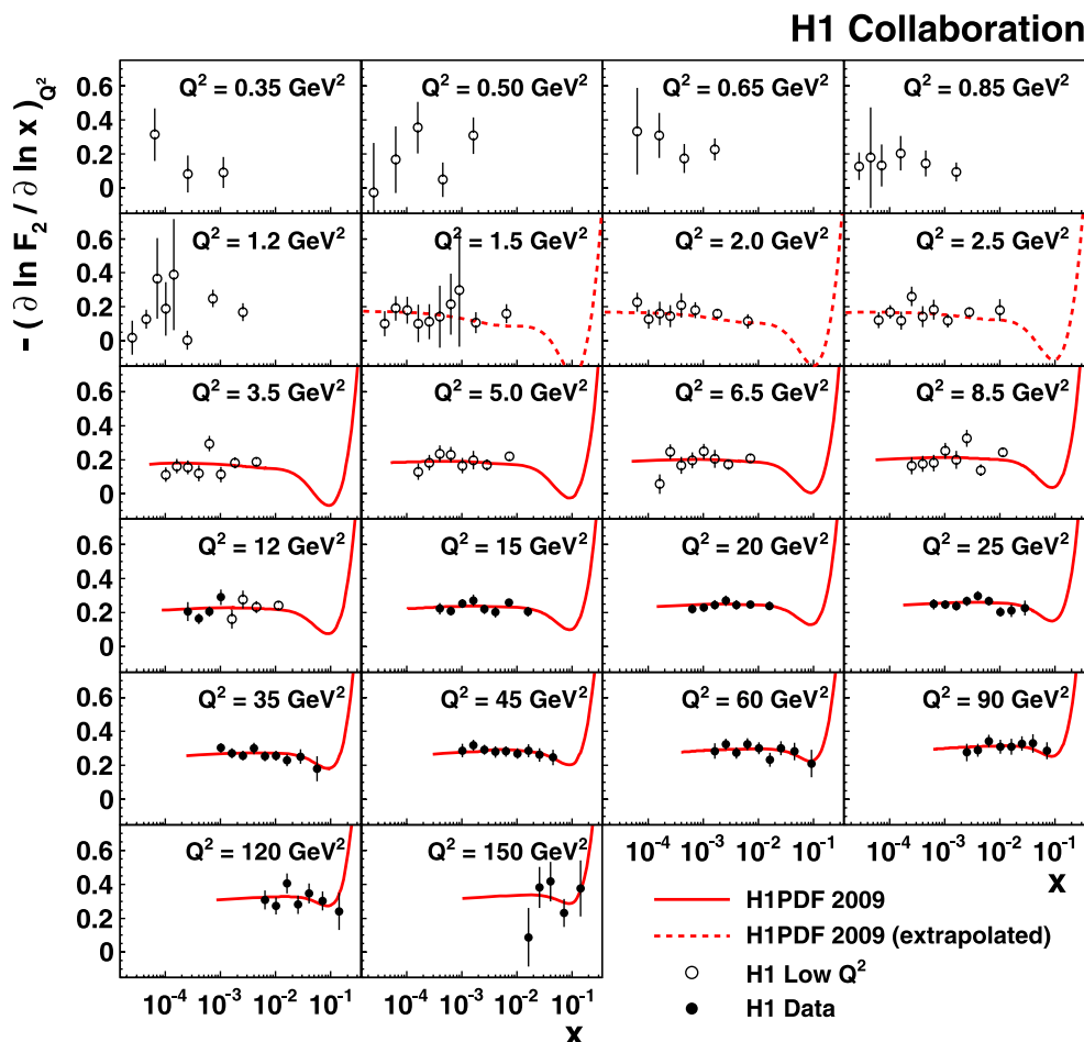
Fig. 8 Measurement of the function \lambda(x, Q^2) , defined as the negative logarithmic x derivative of \ln F_2 as a function of x at various values of Q^2 . The data of this measurement (closed circles) are complemented with the published data at lower Q^2 (open circles) [2]. The error bars represent the total measurement uncertainties. The solid curve represents the prediction of the QCD fit for Q^2 \geq 3.5 \text{ GeV}^2 , which is also shown extrapolated down to Q^2 = 1.5 \text{ GeV}^2 (dashed)
