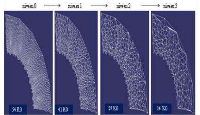
Figure 8 : example of two fragments simplification with maximum radius of curvature = 120°.
