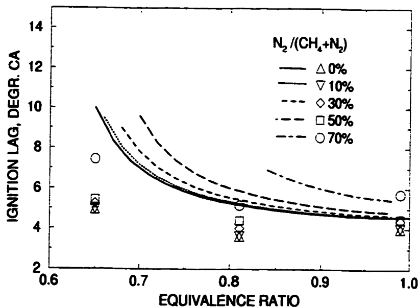
Figure 6.6: The Variation of Ignition Lag Period in a CFR Engine Fueled with Methane-Nitrogen Mixtures for Different Equivalence Ratios at a Compression Ratio of 8.5:1, Spark Timing of 20^\circ BTC, Intake Charge Temperature of 294 K and Atmospheric Pressure. The Corresponding Experimental Data are also Shown.
