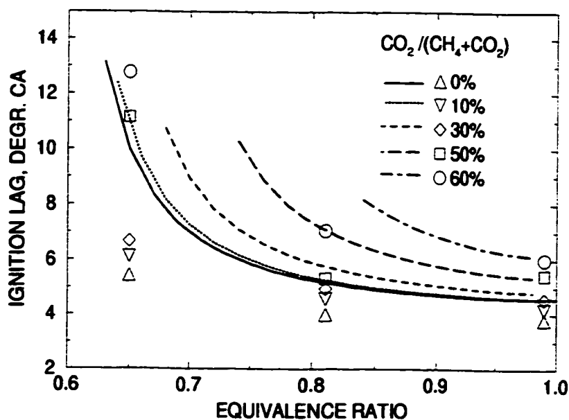
Figure 6.7: The Variation of Ignition Lag Period in a CFR Engine Fueled with Methane-Carbon Dioxide Mixtures for Different Equivalence Ratios at a Compression Ratio of 8.5:1, Spark Timing of 20^\circ BTC, Intake Charge Temperature of 294 K and Atmospheric Pressure. The Corresponding Experimental Data are also Shown.
