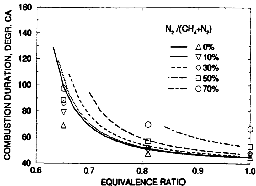
Figure 6.3: The Variation of Combustion Duration in a CFR Engine Fueled with Methane-Nitrogen Mixtures for Different Equivalence Ratios at a Compression Ratio of 8.5:1, Spark Timing of 20^\circ BTC, Intake Charge Temperature of 294 K and Atmospheric Pressure. The Corresponding Experimental Data are also Shown.
