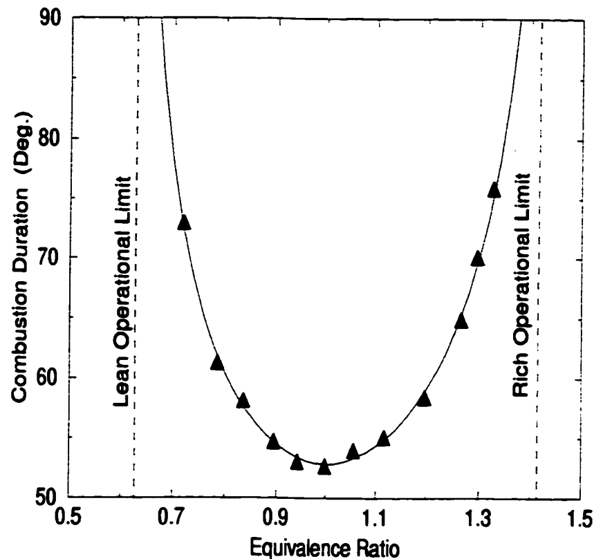
Figure 3.2: Typical Variations of Experimentally Derived Combustion Duration Versus Equivalence Ratio in a CFR Spark Ignition Engine with Methane at 900 rev./min., \theta_{st} = 10 BTDC, CR = 8.5:1 , T_o = 300 K and P_o = 87 kPa.
