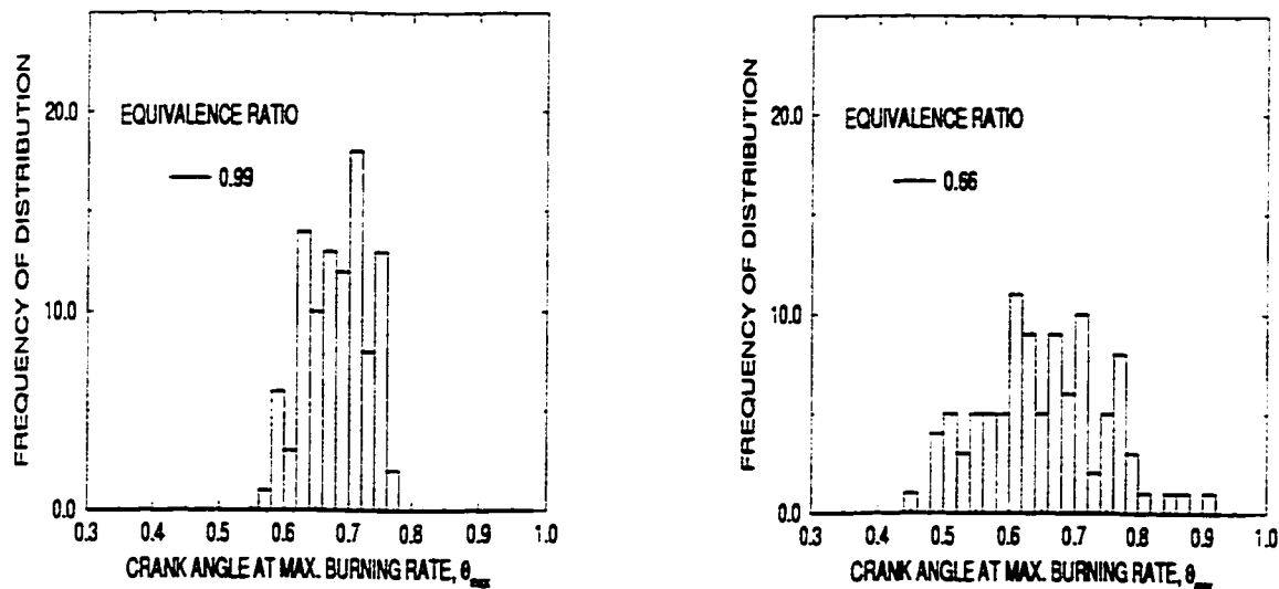
Figure 8.7: The Frequency of Distribution of Normalized Crank Angle at Maximum Burning Rate, \theta_{max} for Different Equivalence Ratios at a Compression Ratio of 8.5:1, Spark Timing of 20 degrees BTC and Initial Temperature of 294 K.
