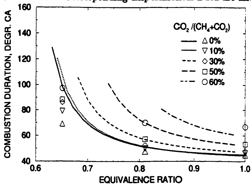
Figure 6.4: The Variation of Combustion Duration in a CFR Engine Fueled with Methane-Carbon Dioxide Mixtures for Different Equivalence Ratios at a Compression Ratio of 8.5:1, Spark Timing of 20^\circ BTC, Intake Charge Temperature of 294 K and Atmospheric Pressure. The Corresponding Experimental Data are also Shown.
