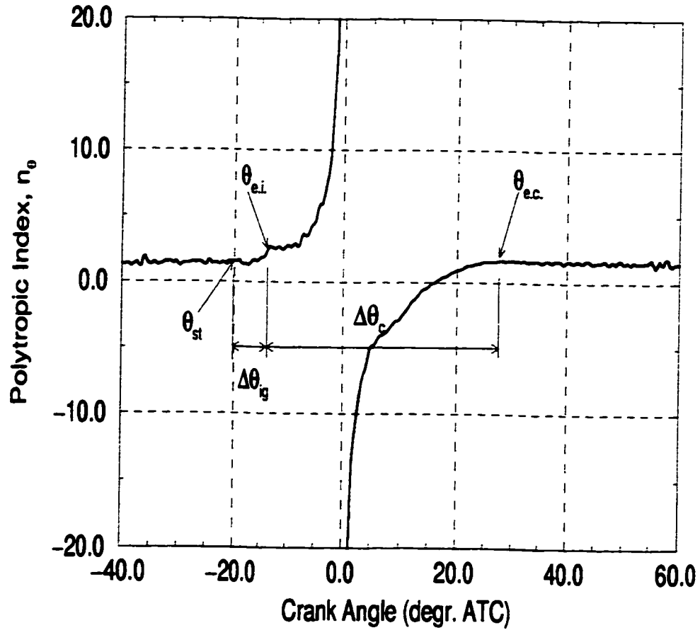
Figure 4.2: The Typical Variation of Polytypic Index with Crank Angle.
