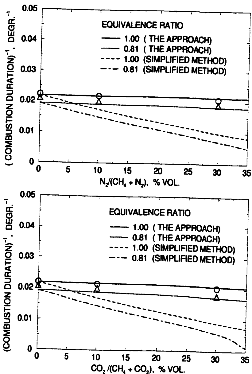
Figure 6.9: The Inverse of Combustion Duration Versus the Concentration of Diluent Present in Fuel Mixture for Different Equivalence Ratios at a Compression Ratio of 8.5:1, Spark Timing of 20^\circ BTC, Intake Charge Temperature of 294 K and Atmospheric Pressure. The Corresponding Experimental Data are also Shown.
