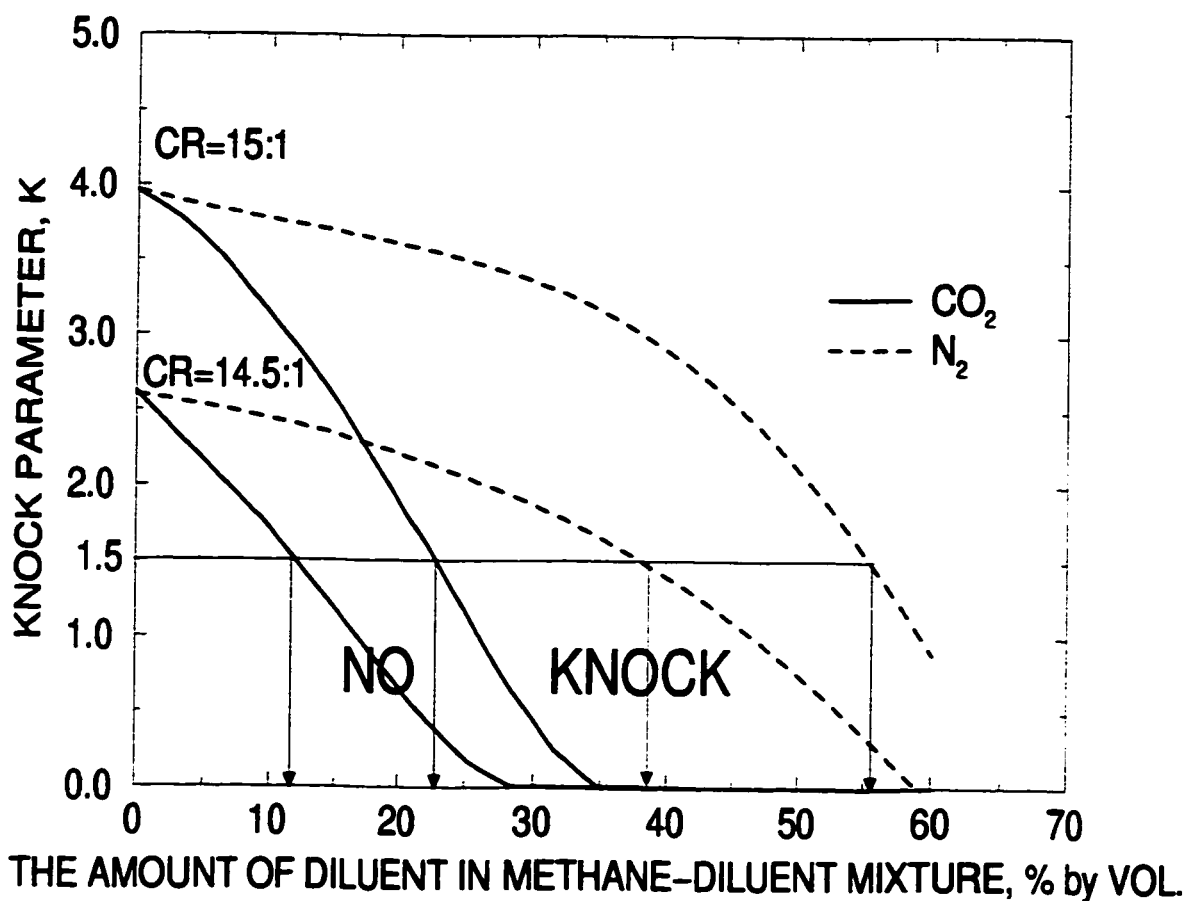
Figure 6.18: The Variation of Knock Parameter, K, Versus Concentration of Various Diluents in Fuel and Diluent Mixtures for Different Compression Ratios at an Equivalence Ratio of 0.90, Spark Timing of 20° BTC, Intake Charge Temperature of 294 K and Atmospheric Pressure.
