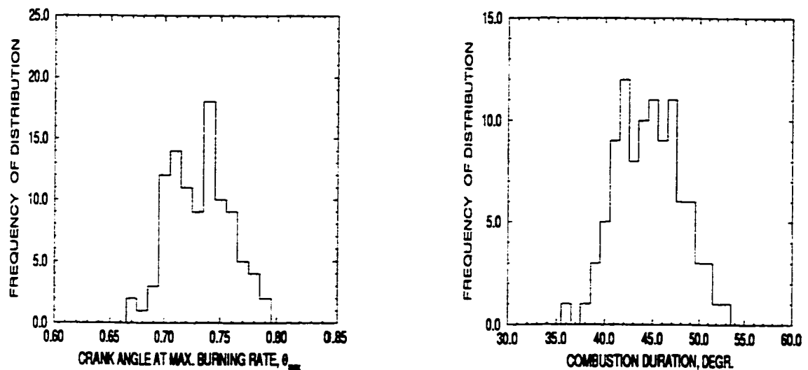
Figure E.3: The Frequencies of Distribution of the Normalized Crank Angle at Maximum Burning Rate, \theta_{max} , and the Combustion Duration, \Delta\theta_c , for 100 Cycles at Equivalence Ratio of 1.10, Compression Ratio of 8.5:1, Spark Timing of 20 degrees BTC and Initial Temperature of 294 K ( Data Set No. 4).
