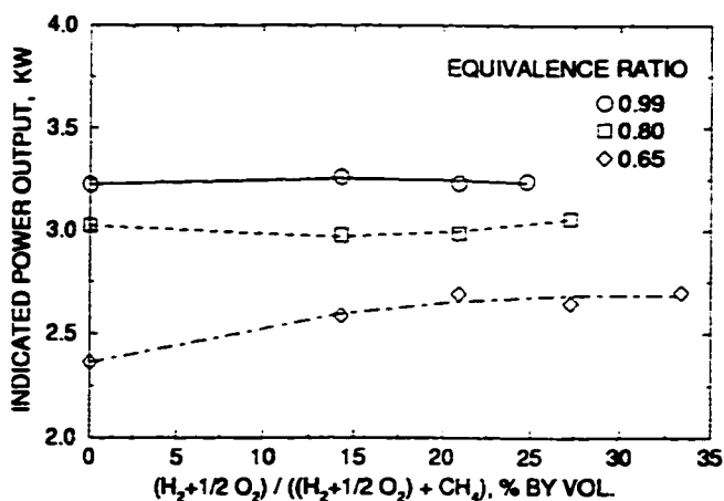
Figure 7.13: The Experimental Indicated Power Output Variations with Concentration of Hydrogen and Oxygen (as the Products of Electrical Dissociation of Water) to Methane for Various Equivalence Ratios at a Compression Ratio of 10:1, Spark Timing of 15 BTC and Initial Mixture Temperature of 294K.
