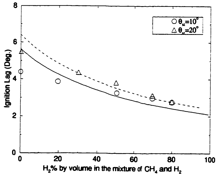
Figure 3.7: Comparison of the Calculated Ignition Lag with Experimental Data for Mixtures of CH_4 and H_2 at 900 rev./min., CR = 8.5:1 , \phi = 1.0 , P_o = 87 kPa, T_o = 300 K.
