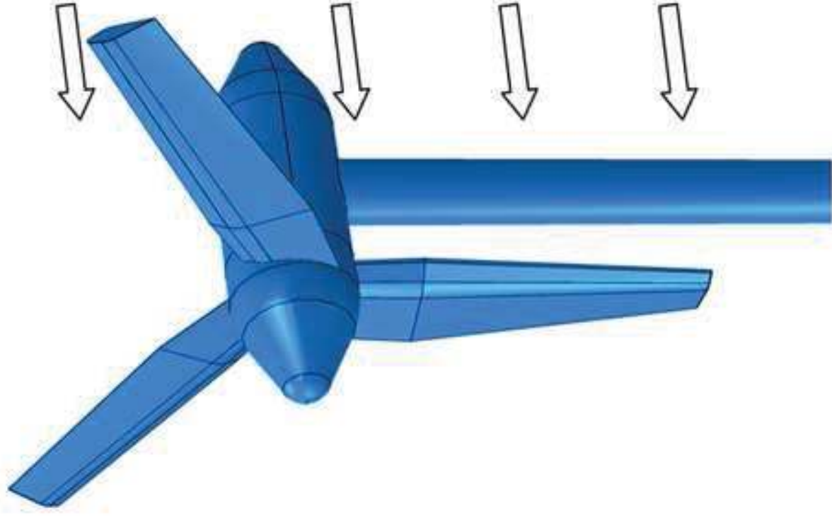
Figure 9 Tower shadow effect on downstream 3 bladed tidal turbine
