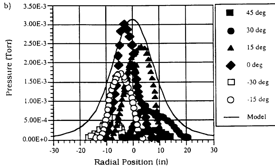
Figure 17: Impact pressure probe data at various angles vs. radial position at axial positions 53 [a)] and 64 cm [b)] from the nozzle exit.
