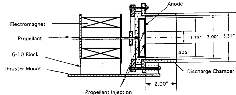
Figure 3: Schematic diagram of the 500 W end-Hall thruster.
