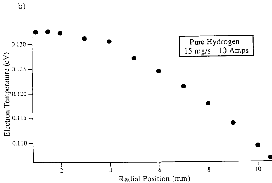
Figure 13: Boltzmann plot of excited states, and corresponding Electron temperature vs. radius with H_2 propellant.
