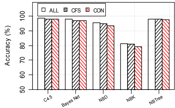
Figure 2: Accuracy of algorithms using CFS subset, CON Subset and All features.
