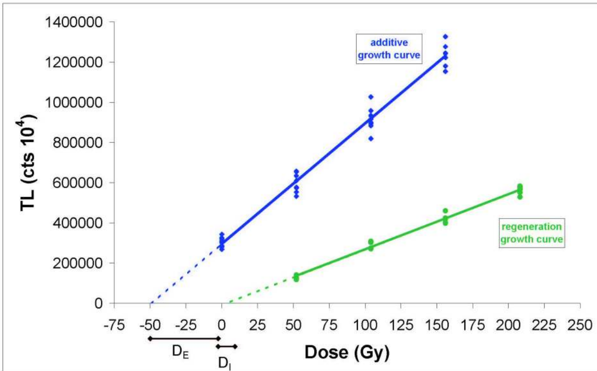
Figure 10. Additive and regeneration growth curves for sample PA-091. The sum of the absolute values of the extrapolation of both data sets to the x-axis essentially gives the palaeodose.
