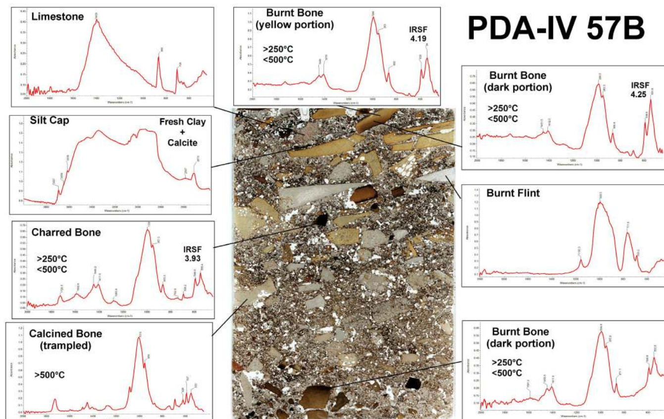
Figure 20. Thin section (PDA-IV 57B) from Layer 8 (Sq G14 X:1002.630; Y:1008.146; Z~6.85) and FT-IR spectra of several particles collected in situ in ATR and Transmission mode.
