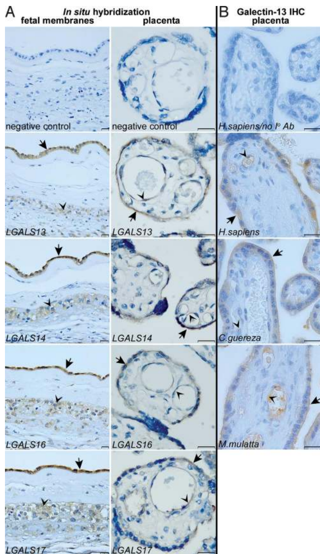
Fig. 2. Chr19 cluster galectins have a similar expression pattern at the maternal-fetal interface. (A Left) In situ hybridization reveals LGALS13 , -14, -16, and -17 expression in the amnion (arrows) and chorionic trophoblasts (arrowheads) in fetal membranes of nonlaboring women. (Right) In the placenta, these genes are predominantly expressed by the syncytiotrophoblast (arrows) and fetal endothelia (arrowheads). (B) Galectin-13 immunostaining is conserved in the syncytiotrophoblast, its apical membrane (arrows), and the endothelia (arrowheads) of human and anthropoid primate placentas. (Scale bars: 20 \mu m.)
