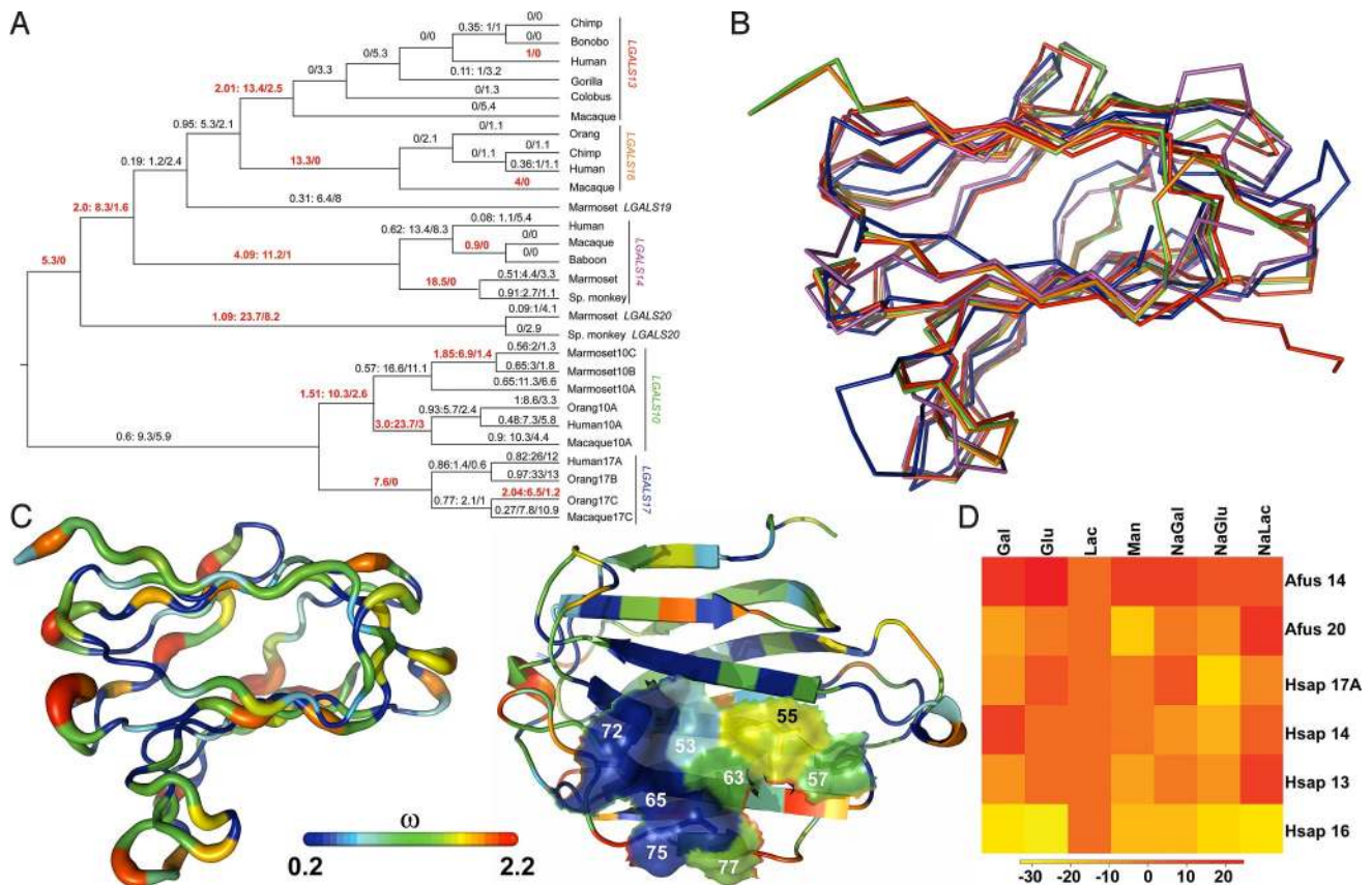
Fig. 4. Evolutionarily changes leading to structural and functional diversification in Chr19 cluster galectins. ( A ) Numbers above the branches of the gene tree represent \omega , N^*dN (nonsynonymous substitutions), and S^*dS (synonymous substitutions), respectively, shown in red on branches with evidence for positive selection. ( B ) Superposition of human galectin structures (10, green; 13, red; 14, purple; 16, orange; 17, blue) demonstrates their conserved \beta -sandwich structure composed of 2 antiparallel sheets. Loop regions show more structural variability. ( C Left ) The width of the ribbon representing the molecular backbone of galectin-16 varies in proportion with site-specific \omega values for all cluster galectins. \omega , also indicated by color spectrum depicted on the bar, is the smallest along \beta -strands and highest in loop regions. ( Right ) The same color coding shows that 4 residues in the CRD of cluster galectins (residues 53, 65, 72, and 75) are under strong purifying selection, others on the opposite side (residues 55, 57, 63, and 77) show more variability. ( D ) Heatmap shows the percentage of competitively eluted proteins from lactose-agarose beads relative to lactose.
