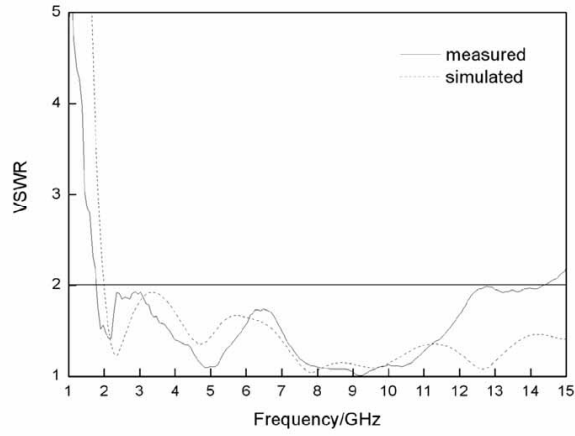
Figure 5. Measured and simulated VSWR of the proposed antenna.
