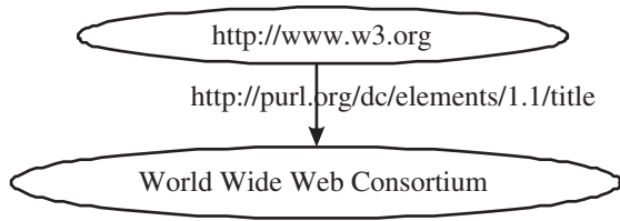
Fig. 1. RDF Graph Example
