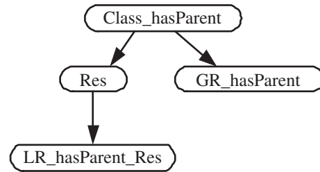
Fig. 4. Class by Local Value Constraint
