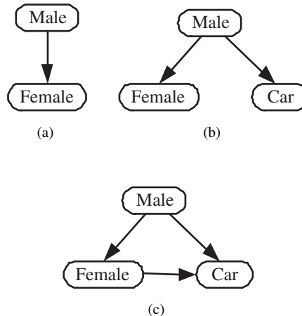
Fig. 8. Class by "owl:disjointWith" Axiom
