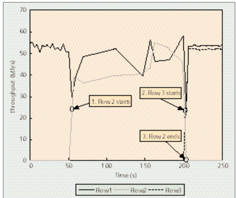
Figure 6. Load-sensitive rerouting results.
