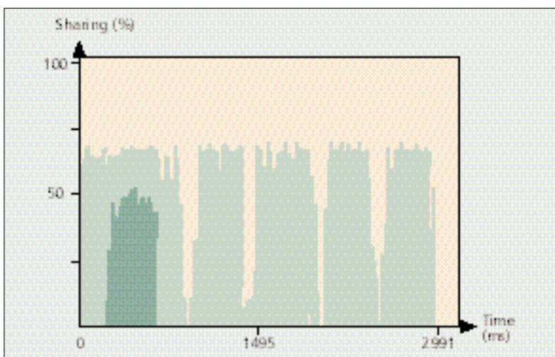
■ Figure 4. Bandwidth sharing between video and FFT streams.
