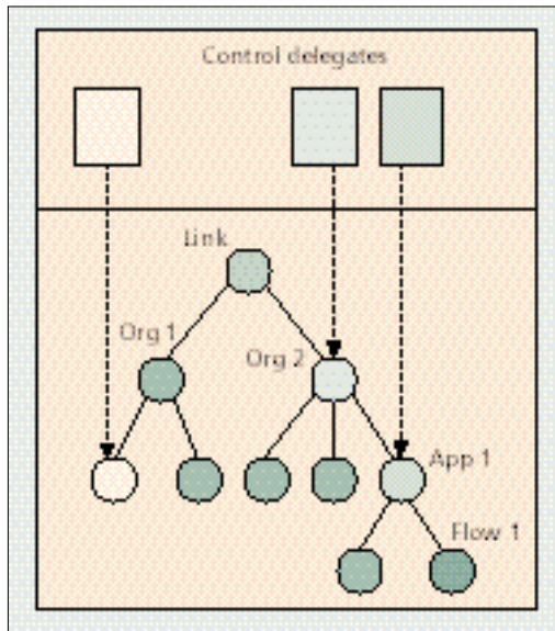
■ Figure 2. Pairing customization in the control and data plane.
