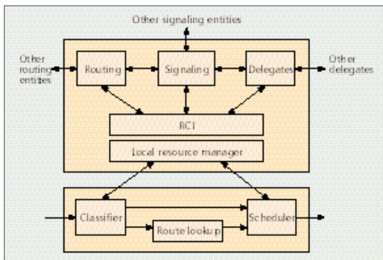
Figure 1. Node architecture.
