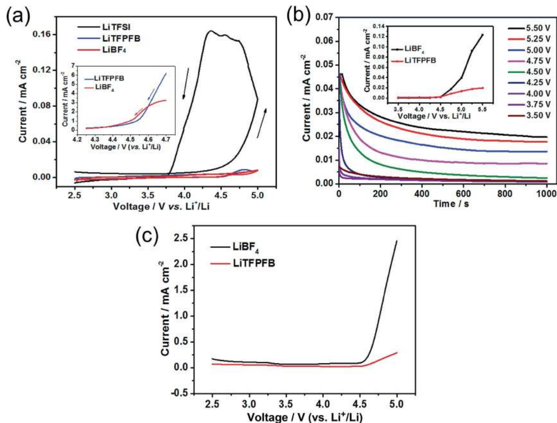
Fig. 3 (a) Cyclic voltammogram curves of 1.0 M LiTFSI/PC, 1.0 M LiBF 4 /PC, and 1.0 M LiTFFPB/PC at a scan rate of 5 mV s -1 using Al as the working electrode and lithium foil as both the counter and reference electrodes. (b) Time-decaying current density of LiTFFPB based cells obtained on an Al electrode at varied potentials vs. Li + /Li (the inset shows the collected current value at 10 3 s vs. voltage). (c) Linear sweep voltammetry scans of 1.0 M LiBF 4 /PC and 1.0 M LiTFFPB/PC on a Pt working electrode at a scan rate of 5 mV s -1 using lithium foil as both the counter and reference electrodes.
