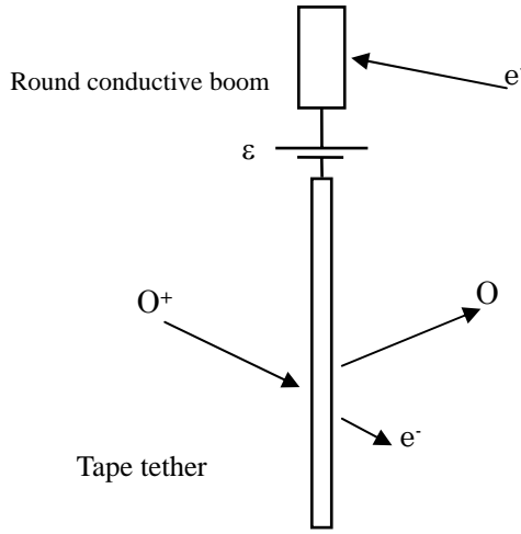
Fig.8-1 Test of the OML theory-1
