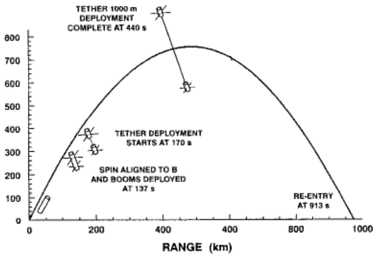
Figure 10 Example of a mission profile for a tether experiment with a sounding rocket (image taken from Oedipus-C mission).
