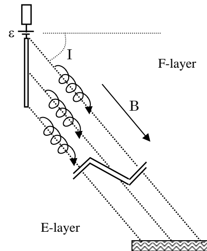
Fig.9 Schematic of beam propagation.
