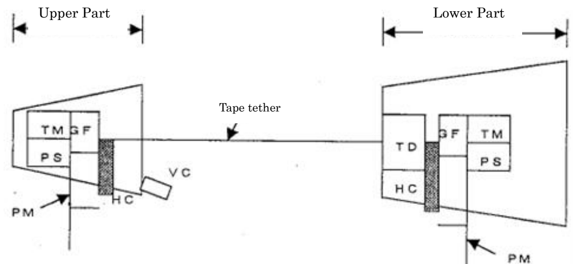
Fig.4 Separation of the payload in the capsule connected by tether
