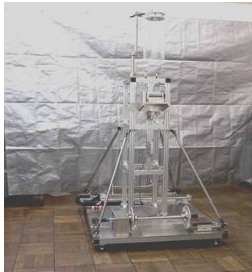
Fig. 11 on-ground experimental device for deployment of tethers with both configurations of string and tape (Tokyo MIT)
