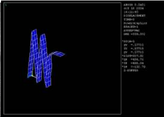
Fig.6 Numerical simulation of deployment
