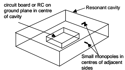
Fig.3 Showing position of small monopoles and circuit board/RC in resonant cavity for test purposes
