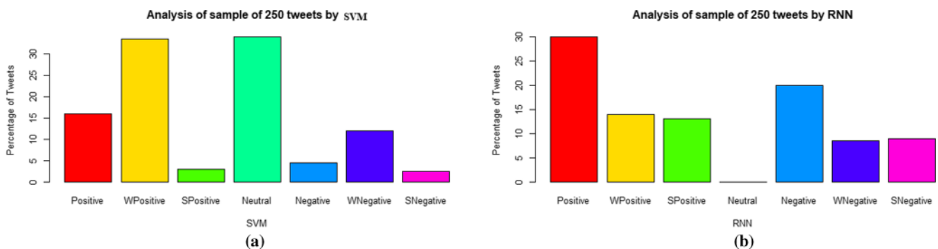
Fig. 10 Analysis of a sample of 250 tweets a SVM result b RNN result
