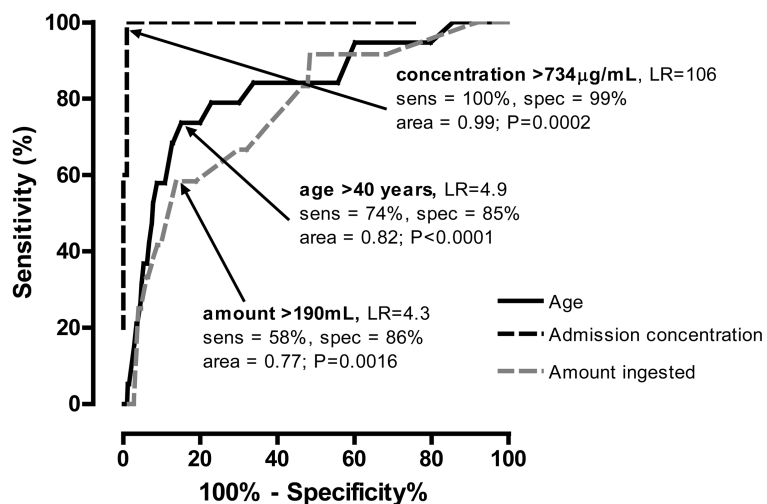
Figure 2. Receiver Operator Characteristic curves demonstrating the prognostic utility* of age, amount ingested and admission glyphosate concentration to predict death * LR is likelihood ratio, sens is sensitivity and spec is specificity
