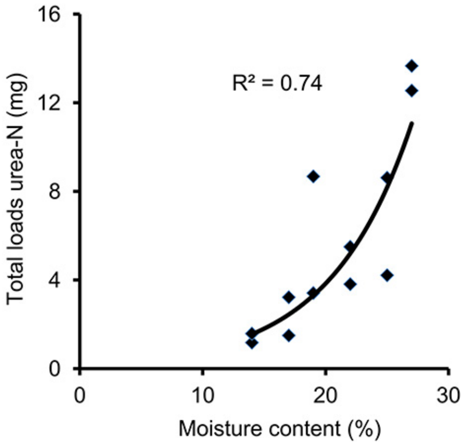
Figure 10. Total load urea-N is positively correlated with antecedent soil moisture content ( R^2 = 0.74 ). The positive relationships between total runoff volume and antecedent soil moisture content and between flow weighted concentration of urea-N and antecedent moisture content combine to result in an exponential relationship ( y = 0.2043 e^{0.0405x} ).
