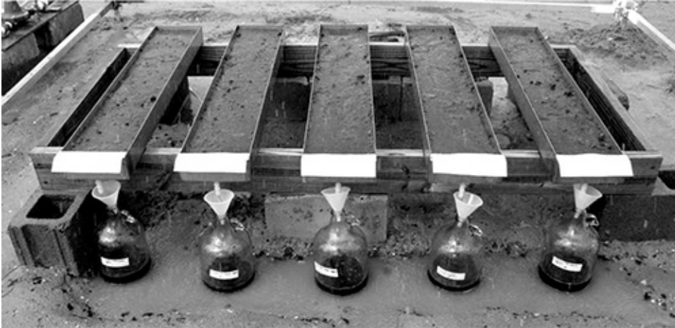
Figure 5. Boxes positioned on the platform for rainfall simulation. Place 5 or 6 boxes in marked positions for each rainfall simulation event. Avoid positioning a box directly under the nozzle to prevent dripping directly onto a box surface.
