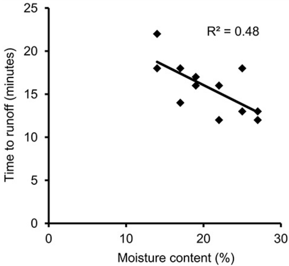
Figure 7. Time to runoff is negatively correlated with antecedent soil moisture content ( R^2 = 0.48 ). The surface of a wet soil saturates quickly. Rainfall that exceeds the hydraulic conductivity of the saturated soil generates runoff.
