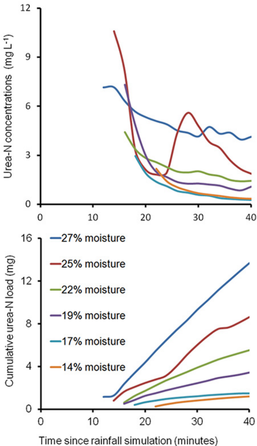
Figure 11. Urea-N concentration and cumulative load relationships over time for one replicate of each antecedent soil moisture content. Although urea-N concentration is not always a smooth function through time, the significant relationships previously discussed can be visualized.
