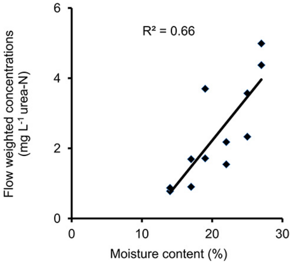
Figure 9. Flow weighted concentration of urea-N is positively correlated with antecedent soil moisture content ( R^2 = 0.66 ). Drier soils allow infiltration that leaches urea-N into the soil and away from the soil surface. When runoff does occur, less urea-N is available at the surface for movement in runoff.
