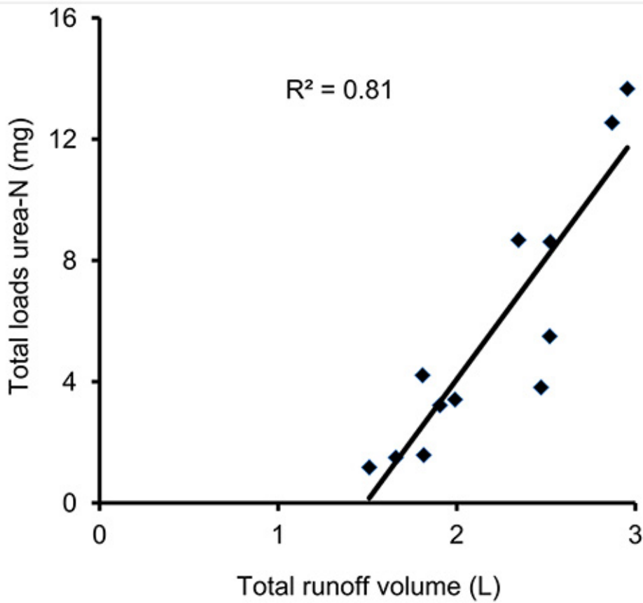
Figure 8. Total load urea-N is positively correlated with runoff volume ( R^2 = 0.81 ). Differences in runoff volume overwhelm differences in concentration of urea-N in runoff.
