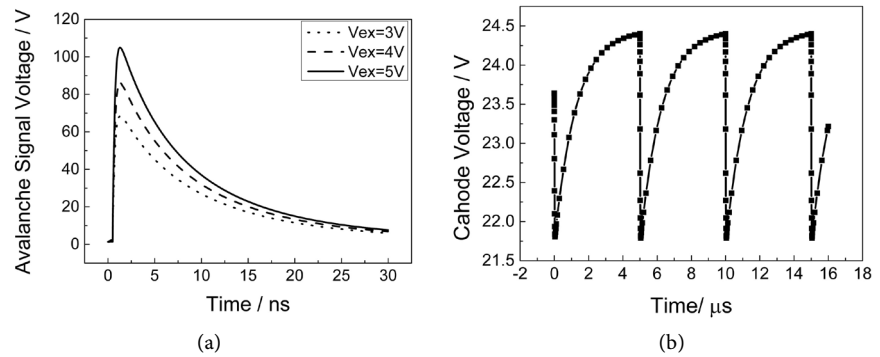
Figure 3. (a) The avalanche signal voltage through R_s at different excess voltage V_{ex} ; (b) The voltage waveform of cathode at the photon pulse frequency of 200 kHz.
