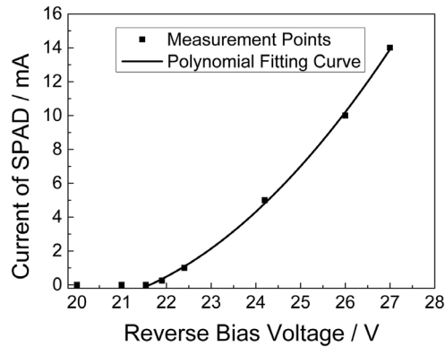
Figure 2. The measurement of I - V characteristic and the 2nd order Polynomial fitting curve.
