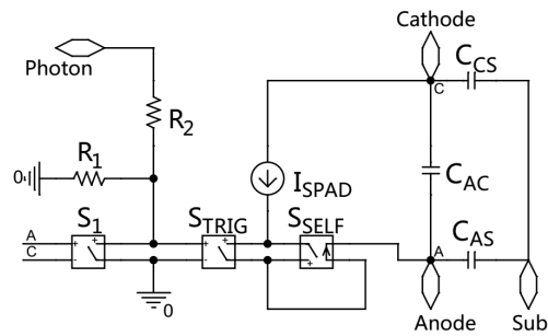
Figure 1. The improved SPAD model. The “Sub” connected to the ground.
