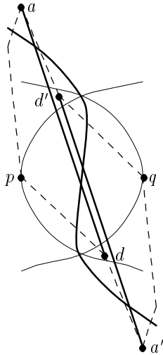
FIG. 14. Although a and d lie on q 's side of the bisector and a' and d' lie on p 's side, ad intersects pq closer to p than a'd' does. This is not possible if the bisector is a line as for the Euclidean metric, see Fig. 4.
