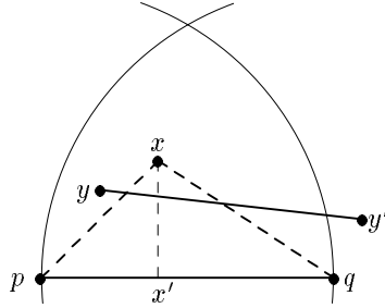
FIG. 6. The quadrilateral xyx'y' is convex because x' \in pq and y, y' \notin pqx .
