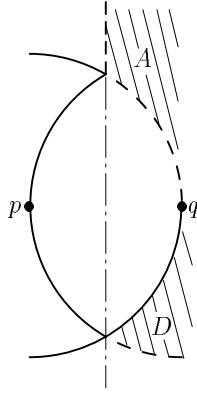
FIG. 3. The regions A and D as defined for the case when a is on the upper chain.
