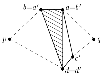
FIG. 5. In the final configuration bd is non-switchable, so a \in A and d \in D , and b'd' is switchable, so Q is type 2. Furthermore, switching b'd' to a'c' increases the degree of b , so a' = b and therefore P and Q overlap in exactly one triangle. The figure ignores that by rights all points should lie outside the lune of pq .
