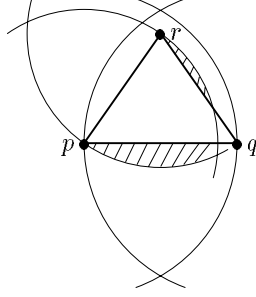
FIG. 9. The points z lie in the interior of \eta_{r\bar{p}} - pqr , which consists of one or two connected components depending on whether or not the angle at r in the triangle pqr is non-acute.
