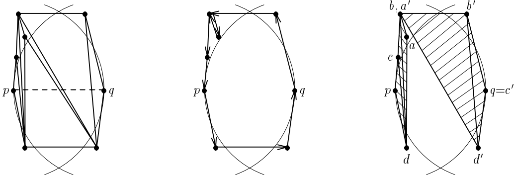
FIG. 1. To the left we see the triangles of t(S) that intersect pq . If we remove the edges intersecting pq we get a polygon whose boundary is oriented in a counterclockwise order. The prefix P and the suffix Q defined for this configuration are illustrated to the right. Although b and a' are the same point, they refer to different angles of this point.
