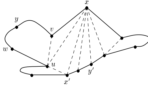
FIG. 8. The polygonal region X is triangulated by fanning out from x , connecting adjacent neighbors of x , and recursing in the thus created pockets. The illustration of this process is schematic and ignores some of the inherent shape constraints for X .
