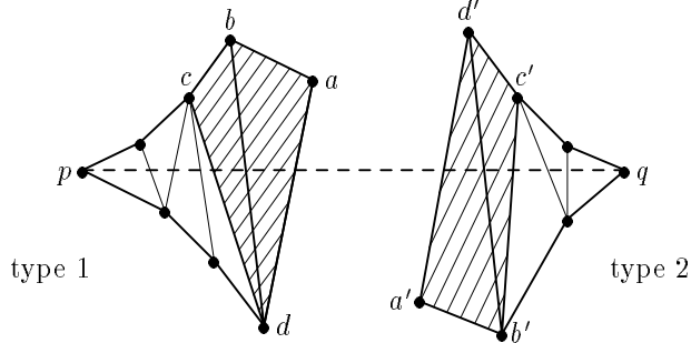
FIG. 2. The prefix P with vertices a, b, c, d and the suffix Q with vertices a', b', c', d' are defined depending on pq . P is type 1 and Q is type 2. For illustration purposes the constraint that all vertices must lie outside the lune of pq has been ignored.
