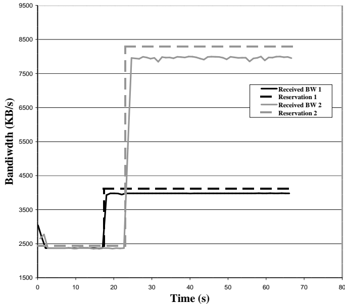
Fig. 4. An example of how our search-based reservation rate strategy determines the correct reservation to use for a TCP application. The application doubled its reservation request twice, then narrowed its reservation with a binary search. The difference between the gross and net reservations is due to packet overheads.
